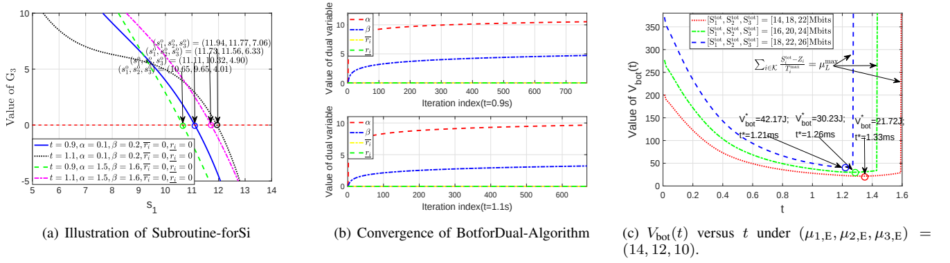
Fig. 2: Illustration of Proposed Algorithm for Solving Problem (EEO-E).
