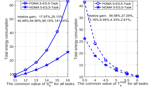
Fig. 6: Comparison between our NOMA-enabled offloading and the FDMA scheme.
