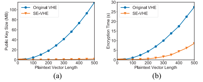
Fig. 2. VHE performance comparison. (a) Public Key Size. (b) Encryption Time.
