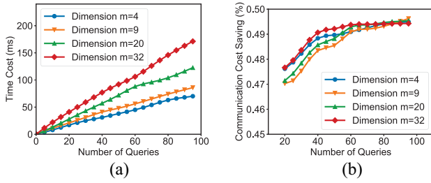
Fig. 3. Performance in SEED- k NN. (a) Time Cost. (b) Communication Overhead.
