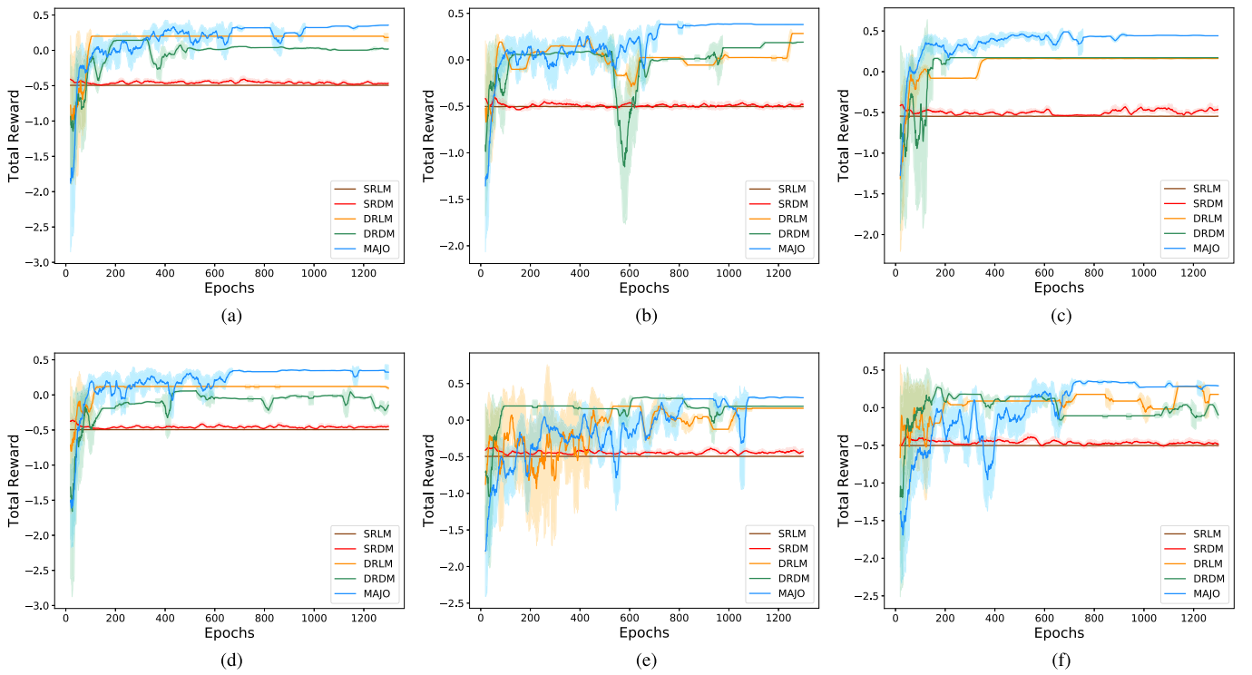
Fig. 7. Performance on total reward. The solid lines are smoothed by window size of 20 epochs, while shaded areas show the standard deviations. (a) b_v(t) = 300 MB, |V| = 30 . (b) b_v(t) = 400 MB, |V| = 30 (c) b_v(t) = 500 MB, |V| = 30 (d) b_v(t) = 200 MB, |V| = 30 (e) b_v(t) = 200 MB, |V| = 40 (f) b_v(t) = 200 MB, |V| = 50 .
