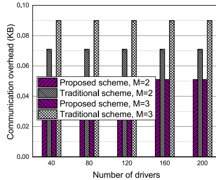
Fig. 10. Communication overhead on RSU-to-TMC communication.
