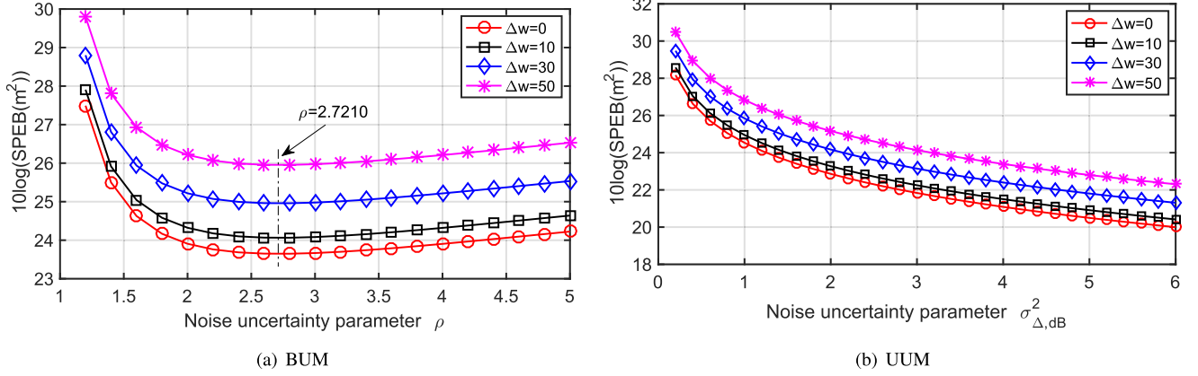
Fig. 6. The worst-case CSPEB versus noise uncertainty parameter \rho or \sigma_{\Delta, \text{dB}}^2 with different warden's position uncertainty \Delta w .
