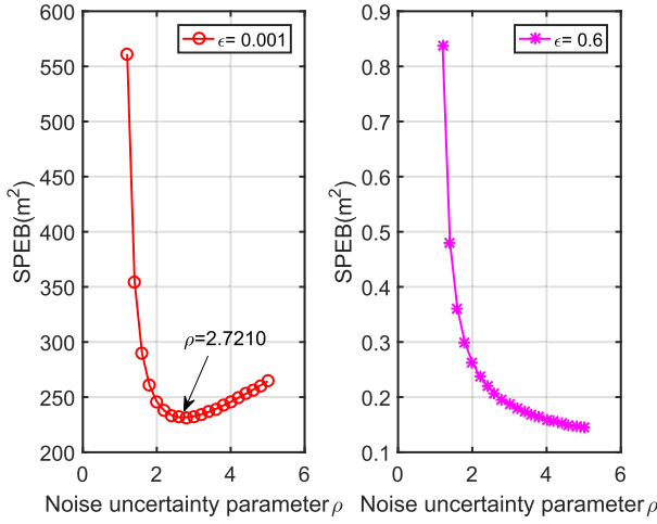
Fig. 3. CSPEB versus noise uncertainty parameter \rho when \epsilon equals to 0.001 and 0.6 respectively in BUM.
