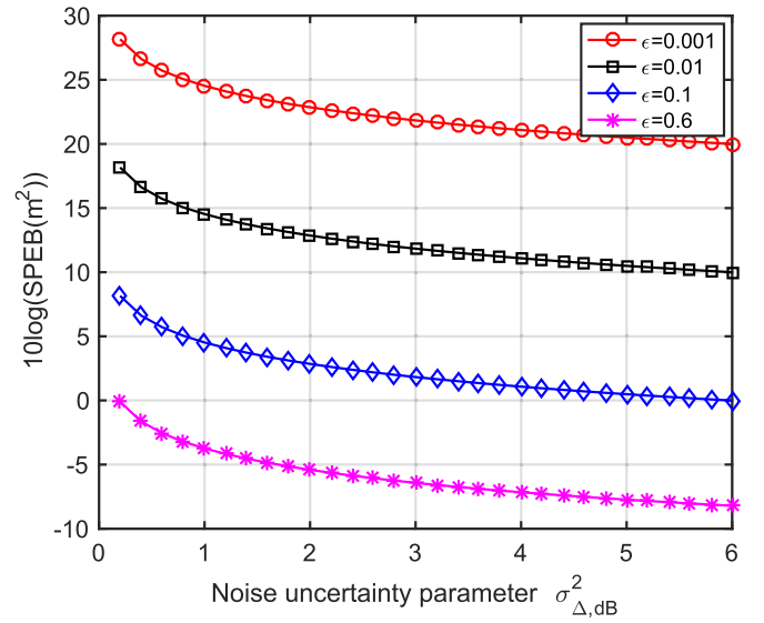
Fig. 5. CSPEB versus noise uncertainty parameter \sigma_{\Delta, \text{dB}}^2 with different covertness requirement coefficient \epsilon in UUM.
