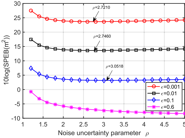
Fig. 4. CSPEB versus noise uncertainty parameter \rho with different covertness requirement coefficient \epsilon in BUM.
