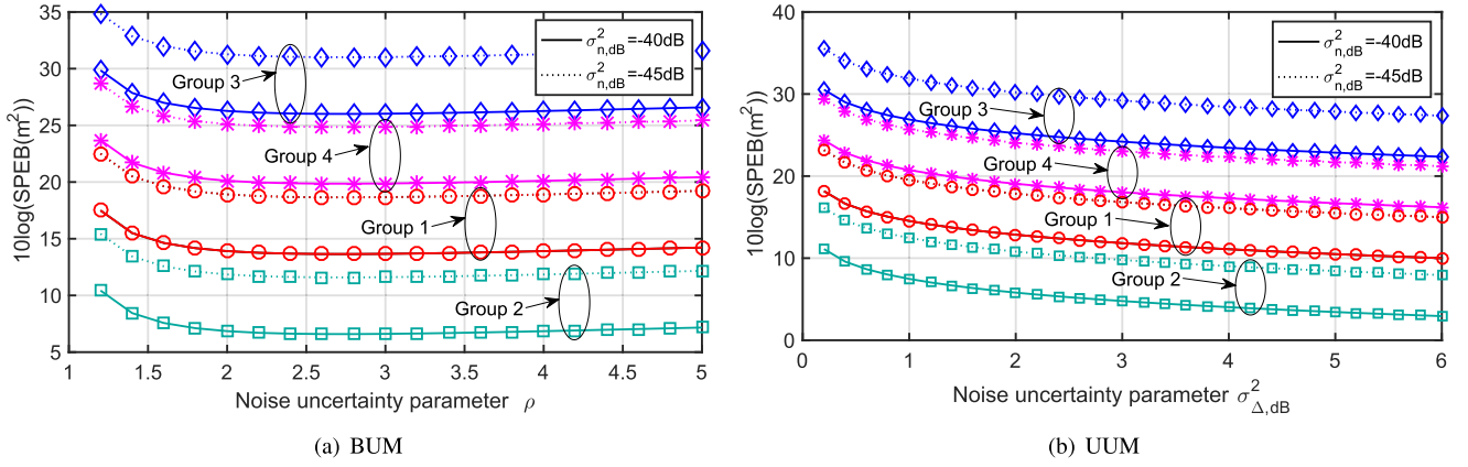
Fig. 7. CSPEB versus noise uncertainty parameter \rho or \sigma_{\Delta, \text{dB}}^2 with different groups (Groups 1-4) of agent and warden and nominal noise power \sigma_{n, \text{dB}}^2 .
