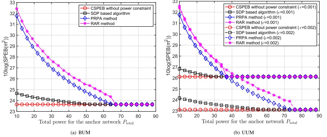
Fig. 8. CSPEB versus the total available power for the anchor network P_{\text{total}} .
