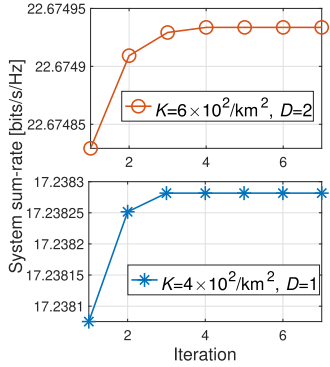
Fig. 6. Convergence of BS clustering algorithm.
