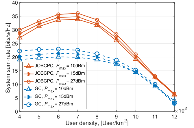
Fig. 17. System sum-rate under different maximum transmit powers P_{\max} versus user density.
