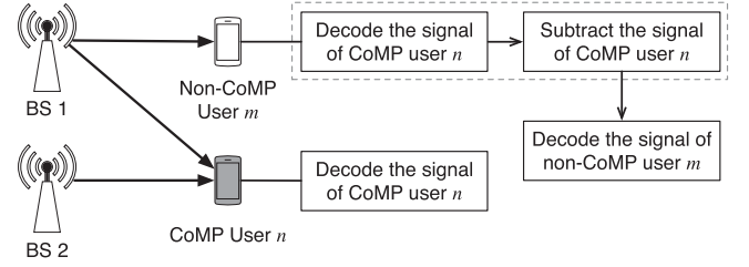
Fig. 2. An illustrative example of NOMA-enabled CoMP transmission.
