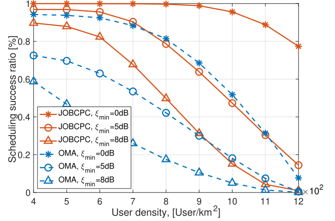
Fig. 16. Scheduling success ratio under different SINR thresholds \xi_{\min} versus user density.
