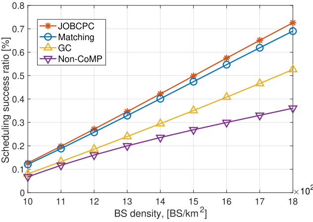
Fig. 10. Scheduling success ratio versus BS density with different schemes.
