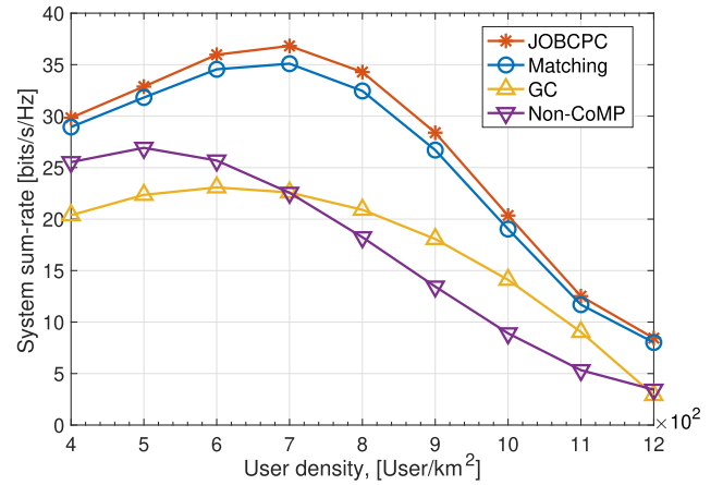
Fig. 7. System sum-rate versus user density with different schemes.
