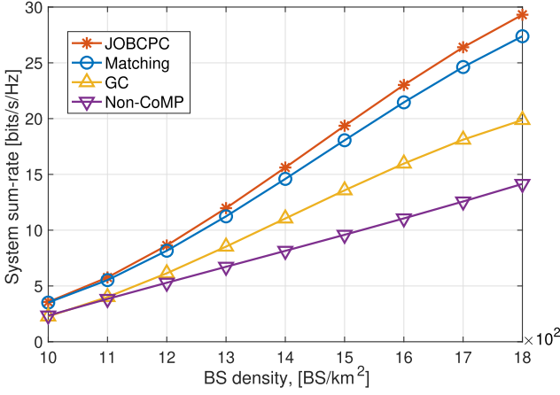
Fig. 9. System sum-rate versus BS density different schemes.
