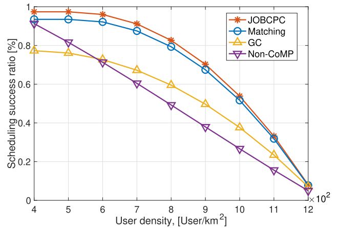
Fig. 8. Scheduling success ratio versus user density with different schemes.
