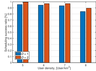
Fig. 14. Scheduling success ratio versus user density with different D .
