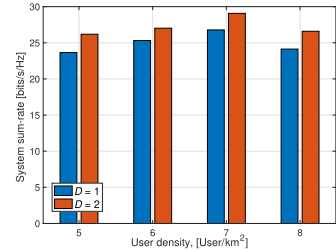
Fig. 13. System sum-rate versus user density with different D .
