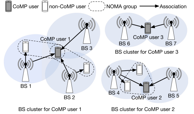
Fig. 1. The BS clusters to perform CoMP transmission in NOMA-UDN, where the CoMP user and non-CoMP user is allowed to coexist in one NOMA group.
