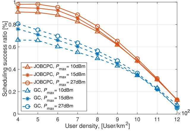
Fig. 18. Scheduling success ratio under different maximum transmit powers P_{\max} versus user density.
