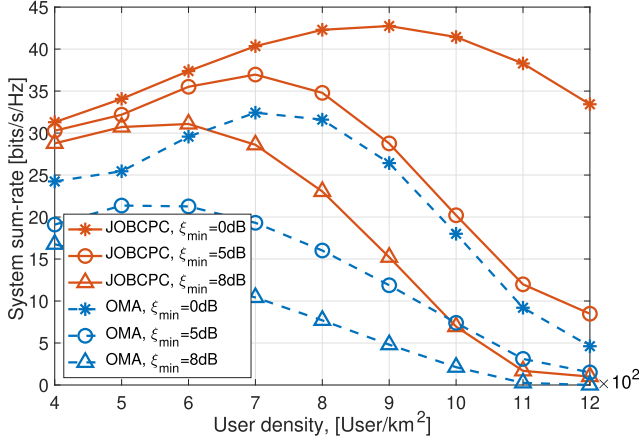
Fig. 15. System sum-rate under different SINR thresholds \xi_{\min} versus user density.
