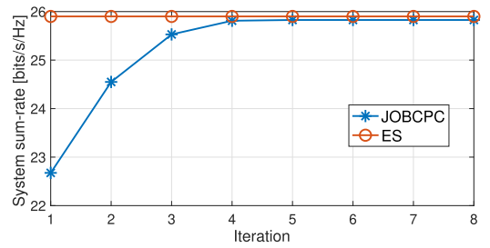
Fig. 4. Convergence of JOBCPC scheme.
