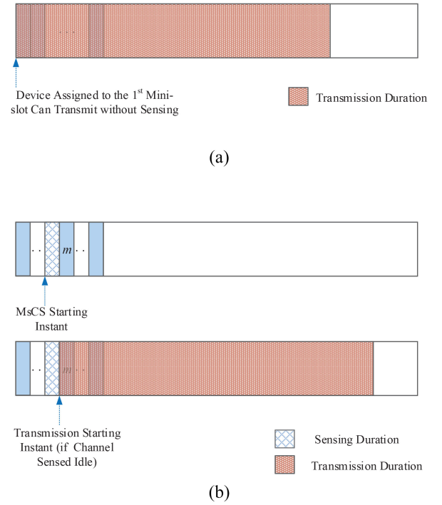
Fig. 3. Illustration of the MsCS. (a) Devices assigned to the first minislot of any slot start transmission immediately when the slot begins, without sensing the channel. (b) Devices assigned to minislot m (> 1) must sense the channel during the (m - 1) th minislot, and start transmission at the beginning of the m th minislot if the channel is sensed to be idle.
