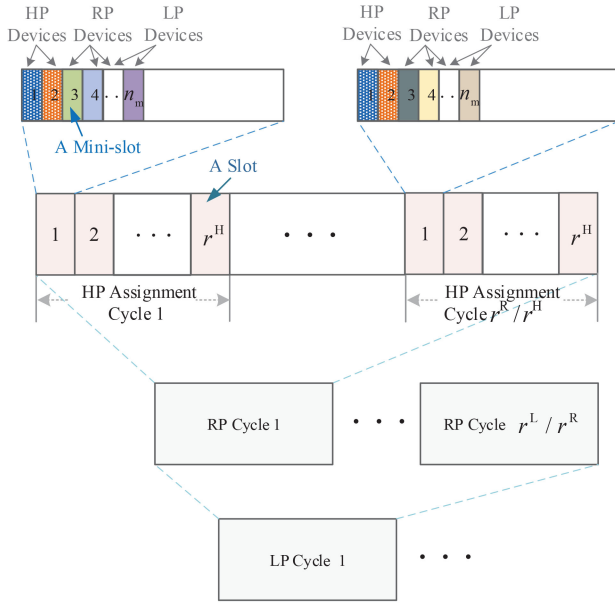
Fig. 5. Illustration of differentiated assignment cycles.
