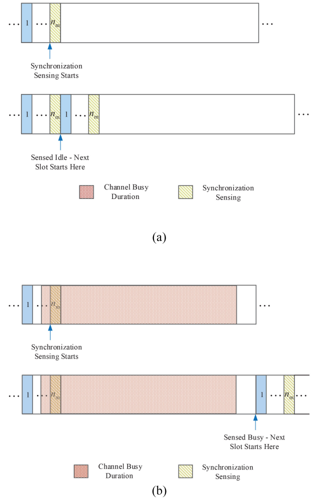
Fig. 4. Illustration of the syncCS. (a) When the last minislot of a slot is sensed idle, the remaining transmission duration of this slot is skipped, and the next slot starts right after the last minislot of this slot. (b) When the last minislot of a slot is sensed busy, the next slot starts after the entire duration of this slot.
