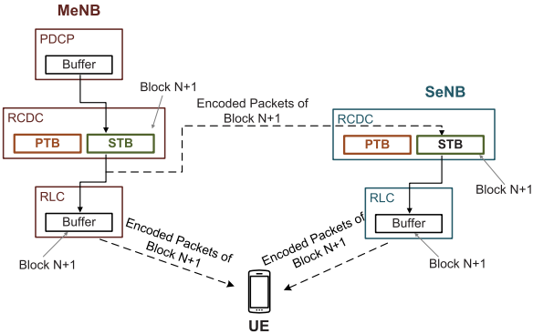
(c) After receiving the ACK, MeNB and SeNB start the transmission of the (N + 1) th block
