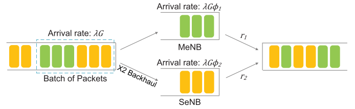
Fig. 5. Queueing models for concurrent transmissions in the conventional DC scheme.
