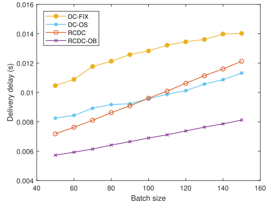
Fig. 14. Average delivery delay with different batch size.
