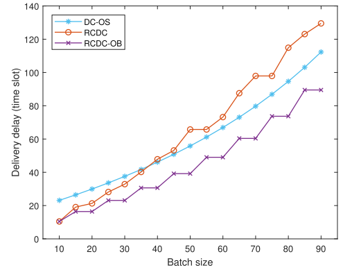
Fig. 11. Average delivery delay under different batch sizes with \lambda = 0.005 , r_1 = 0.2 and r_2 = 0.8 .
