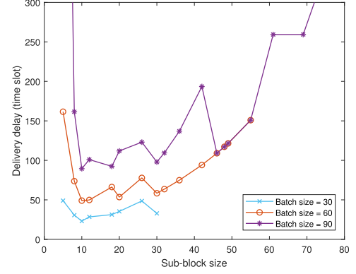
Fig. 8. Average delivery delay with different sub-block size.
