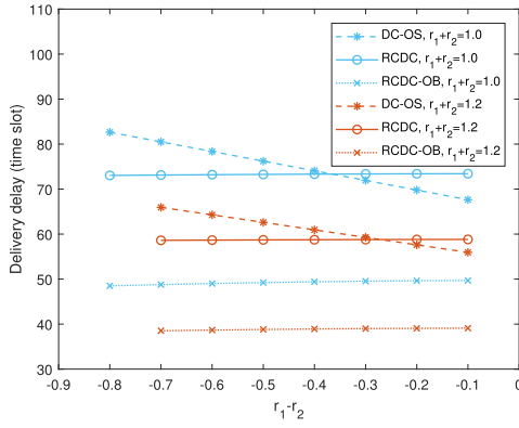
Fig. 9. Average delivery delay under different service rate of eNBs with \lambda = 0.005 .
