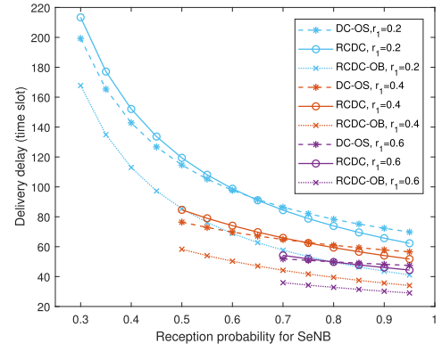
Fig. 10. Average delivery delay under different service rate of eNBs with \lambda = 0.005 .
