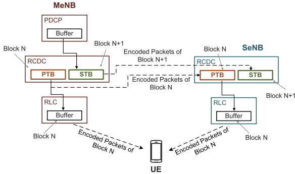
(b) MeNB starts the early encoding of the (N + 1) th block
