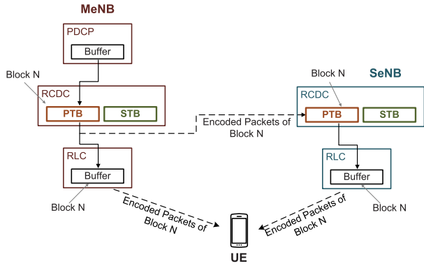
(a) MeNB and SeNB are transmitting the N th block
