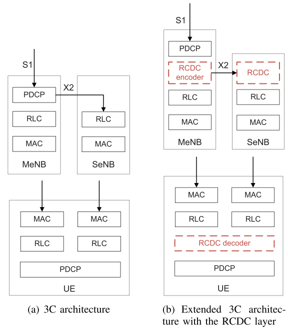
Fig. 2. User plane architectures for dual connectivity architecture.
