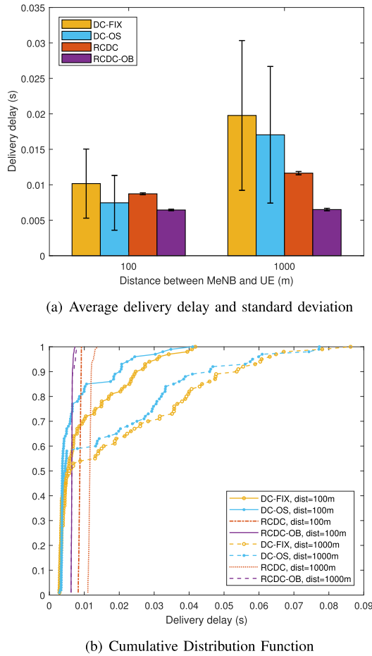
Fig. 15. Delivery delay with different distance between UE and MeNB.
