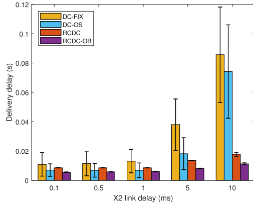
Fig. 13. Average delivery delay and standard deviation under different X2 link latency.
