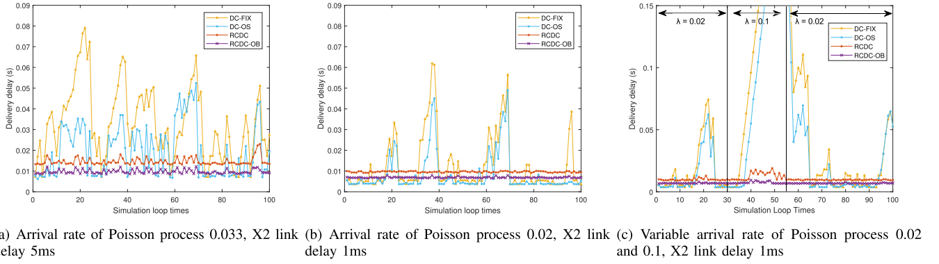
Fig. 12. Instantaneous delivery delay with different schemes.
