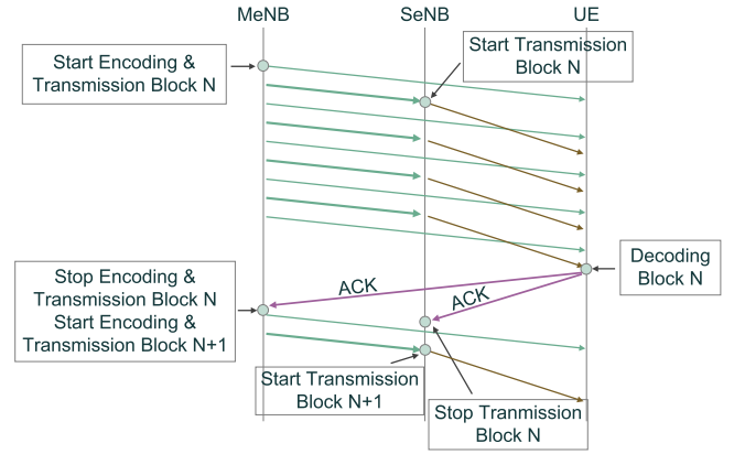
Fig. 3. Flow chart of the encoding, transmission and decoding procedures in the RCDC protocol.
