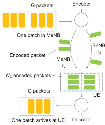
Fig. 6. Queueing models for the RCDC scheme.
