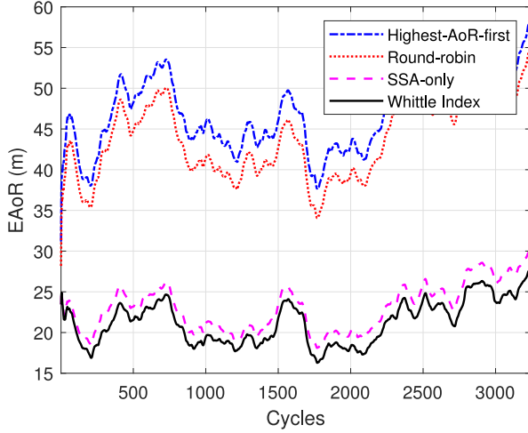
Fig. 9. EoR when the number of computing slots in each cycle, i.e. , K , is 10.
