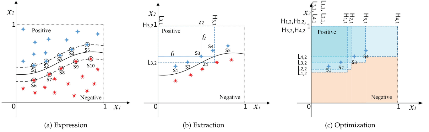
Fig. 2. A simple example of extracting hyper-rectangles from the SVM classifier.
