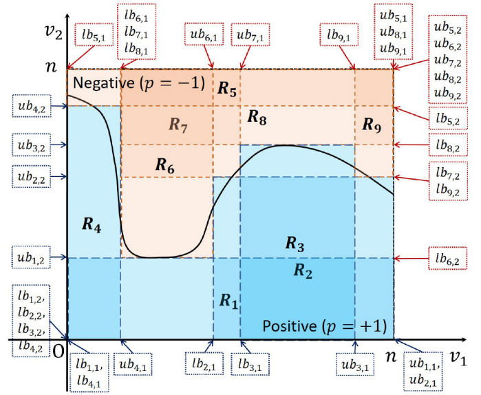
Fig. 2. Example of an SVM classifier and extracted rules.
