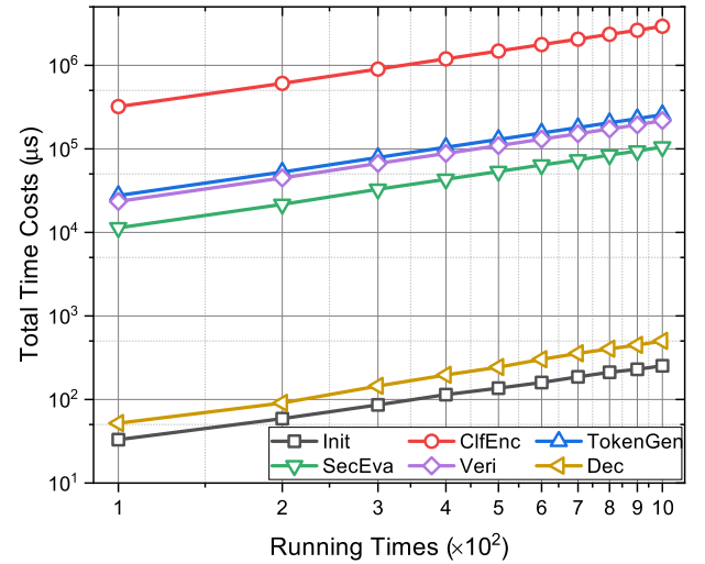
Fig. 6. Total time costs of VSSVMC .
