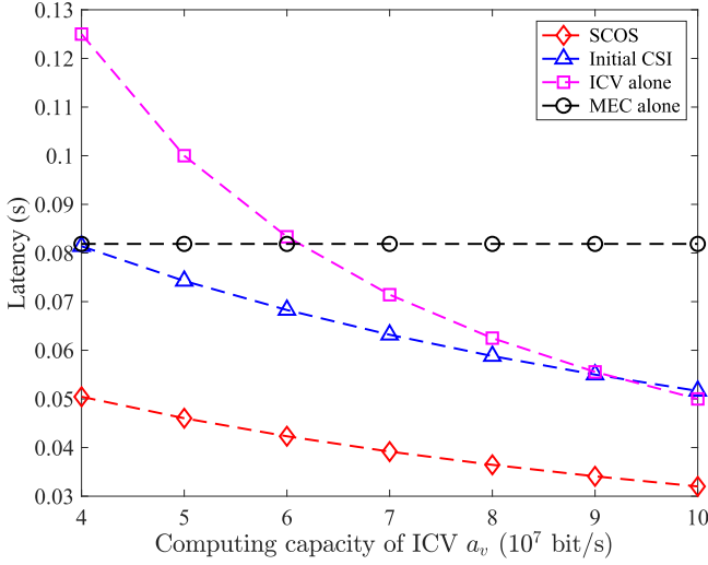
Fig. 5. Latency in terms of ICV computing capacity, i.e., a_v , where we set a_m = 12 \times 10^7 bit/s, N_m = 10 , N_e = 4 , and transmission SNRs of SBS and ICV are 20 dB and 10 dB, respectively.
