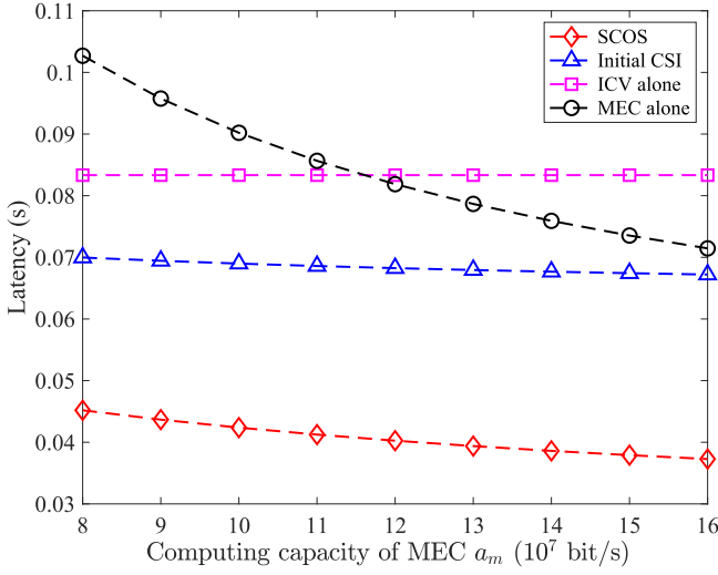
Fig. 4. Latency in terms of MEC server computing capacity, i.e., a_m , where we set a_v = 6 \times 10^7 bit/s, N_m = 10 , N_e = 4 , and transmission SNRs of SBS and ICV are 20 dB and 10 dB, respectively.
