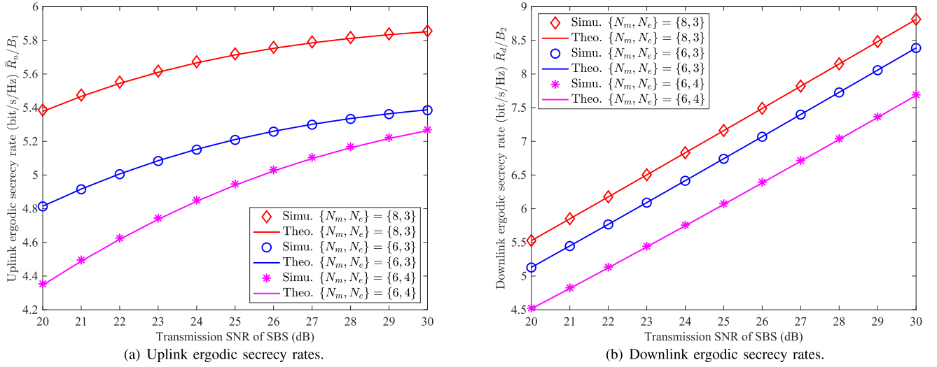
Fig. 2. Numerical results of uplink and downlink ergodic secrecy rates in terms of SBS transmission SNR, where ICV transmission SNR is 10 dB in uplink.
