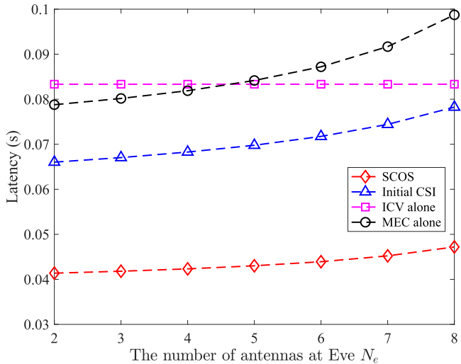
Fig. 9. Latency in terms of the number of antennas at Eve, i.e., N_e , where we set a_m = 12 \times 10^7 bit/s, a_v = 6 \times 10^7 bit/s, N_m = 10 , and transmission SNRs of SBS and ICV are 20 dB and 10 dB, respectively.
