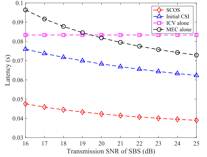
Fig. 6. Latency in terms of transmission SNR of SBS, where we set a_m = 12 \times 10^7 bit/s, a_v = 6 \times 10^7 bit/s, N_m = 10 , N_e = 4 , and transmission SNR of ICV is 10 dB.
