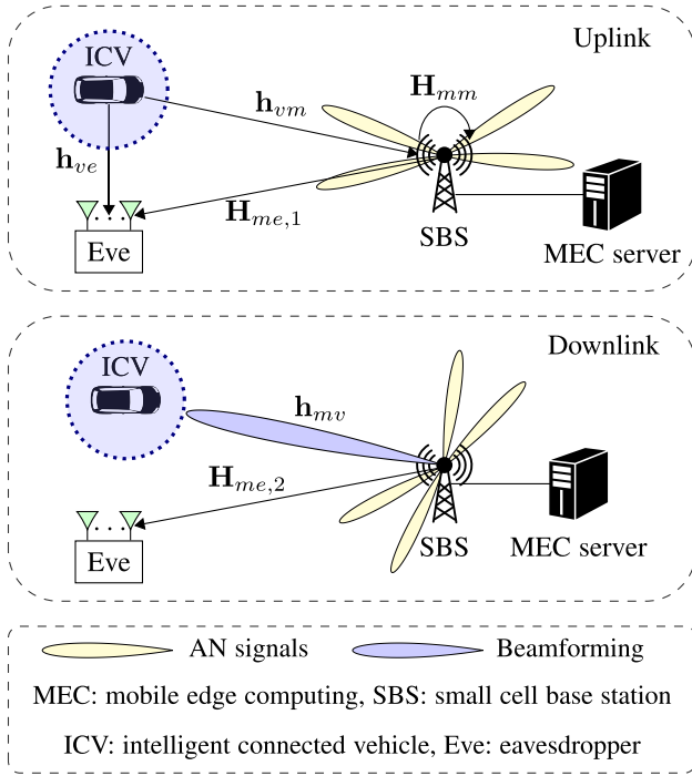
Fig. 1. A communication model with a multiple antenna eavesdropper. An uplink is to upload a part of computation tasks to a nearby SBS. After the MEC server obtains computation results, a downlink is used to download the computation results to the ICV. In addition, beamforming and AN schemes are illustrated in Section IV.
