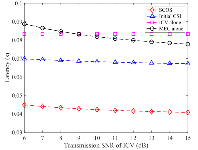
Fig. 7. Latency in terms of transmission SNR of ICV, where we set a_m = 12 \times 10^7 bit/s, a_v = 6 \times 10^7 bit/s, N_m = 10 , N_e = 4 , and transmission SNR of MEC server is 20 dB.
