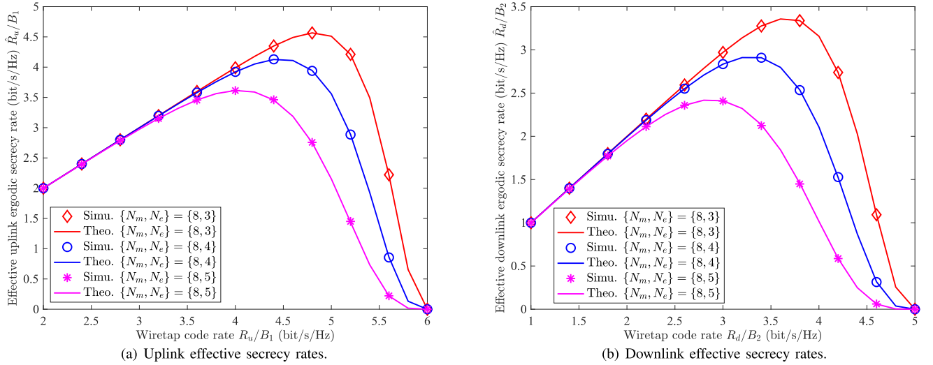
Fig. 3. Numerical results of uplink and downlink effective secrecy rates in terms of wiretap code rates, where transmission SNRs of ICV and SBS are 10 dB and 20 dB, C_{v,u}/B_1 = 6 bit/s/Hz, and C_{v,d}/B_2 = 5 bit/s/Hz.
