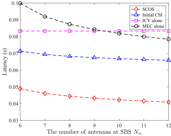
Fig. 8. Latency in terms of the number of antennas at SBS, i.e., N_m , where we set a_m = 12 \times 10^7 bit/s, a_v = 6 \times 10^7 bit/s, N_e = 4 , and transmission SNRs of SBS and ICV are 20 dB and 10 dB, respectively.
