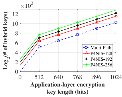
Fig. 8. Cryptographic complexity.
