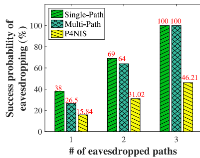
Fig. 7. Difficulties of eavesdropping.
