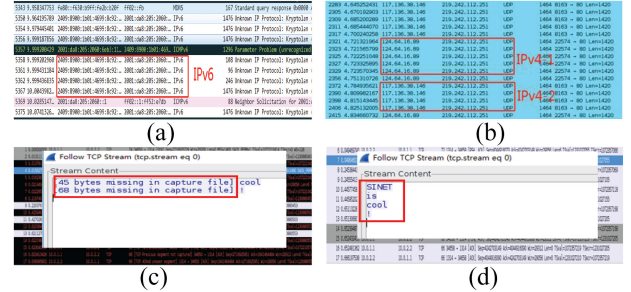
Fig. 10. Snapshots of eavesdropping results. (a) Eavesdropping on one path. (b) Eavesdropping on multiple paths. (c) Eavesdropping on all available paths. (d) Eavesdropping with decryption keys.
