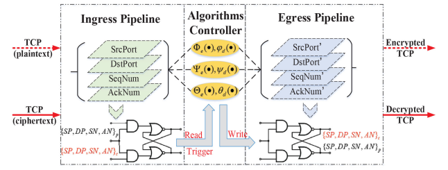
Fig. 3. Programmable cryptographic design.
