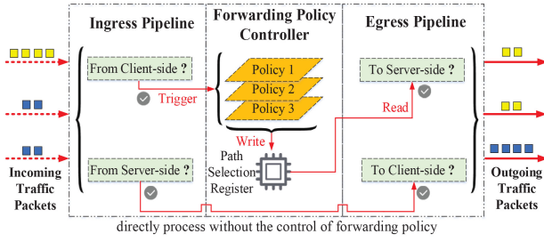
Fig. 2. Programmable forwarding defense.
