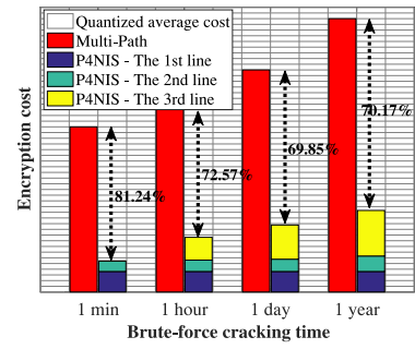
Fig. 9. Encryption cost.
