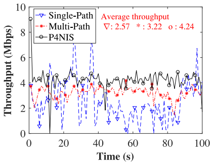
Fig. 14. Transmission throughput.
