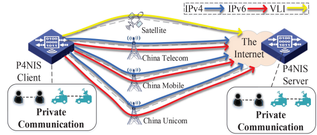
Fig. 6. Typical use case of P4NIS.
