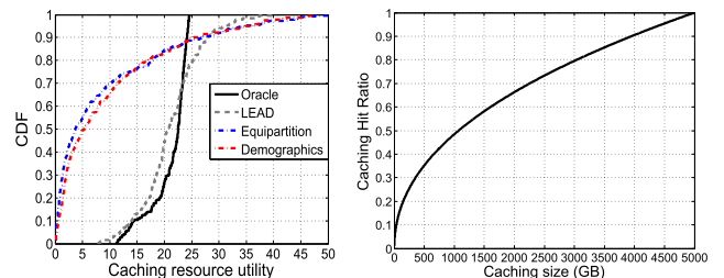
(a) CDFs of caching resource utilities of edge nodes (b) caching hit ratio vs. the cache size in the Zipf distribution
