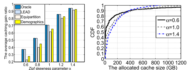
(a) The average caching gain ratio vs. \alpha (b) CDFs of cache size allocations vs. \alpha
