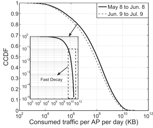
Fig. 3. CCDFs of AP traffic consumption.
