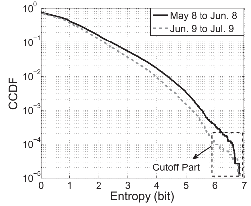
Fig. 4. CCDFs of AP traffic-weighted entropy.
