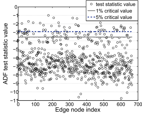
Fig. 14. Comparison between the ADF test statistic and percentile critical value.
