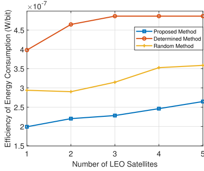
Fig. 7. Efficiency of energy consumption with different L .
