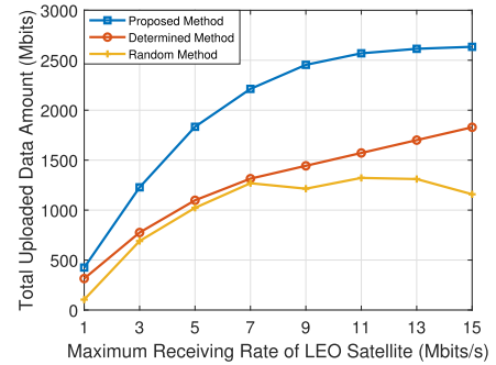
Fig. 6. Total uploaded data amount with different R_{\max} .
