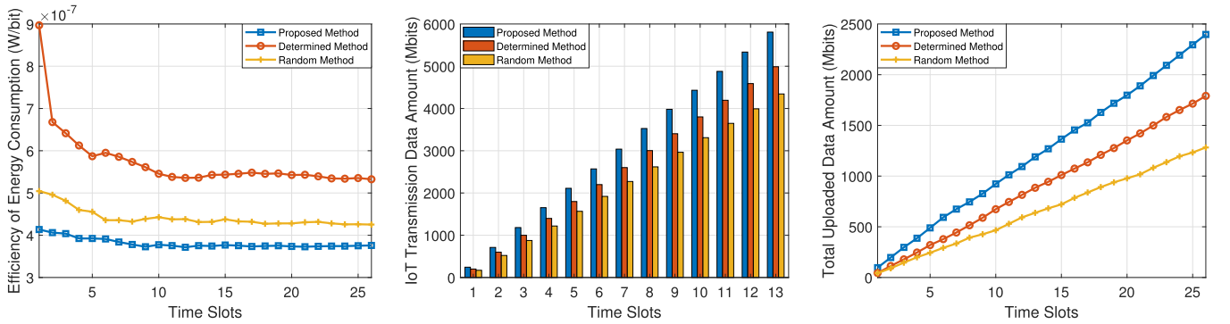
Fig. 3. Performance comparison of three methods: (a) Efficiency of energy consumption (W/bit); (b) IoT transmission data amount (Mbits); (c) Total uploaded data amount of UAVs (Mbits).
