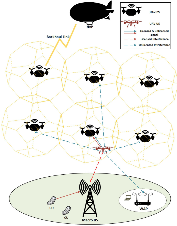
Fig. 1. LTE-U UAV-Cellular network system model.
