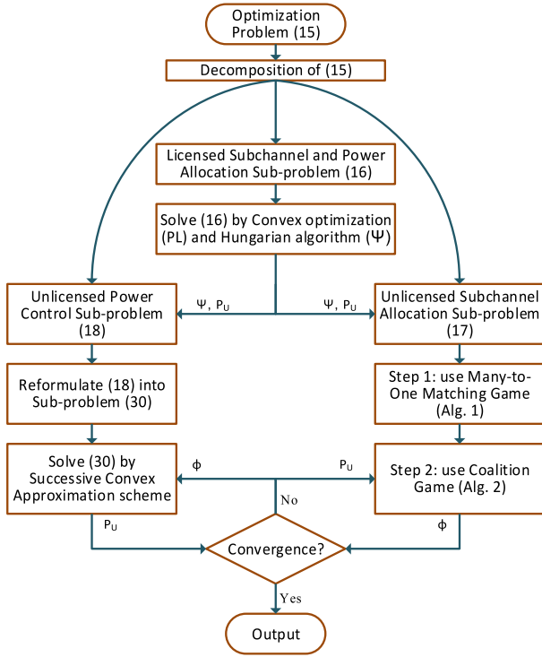
Fig. 2. Solution process of the problem (15).
