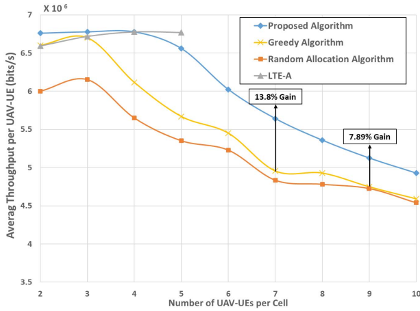
Fig. 4. Average throughput per UAV-UE for different schemes vs. n (number of UAV-UEs per cell).
