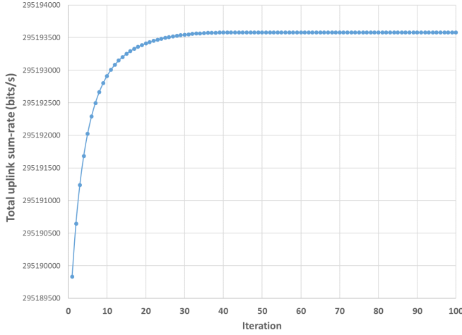
Fig. 7. Convergence of algorithm 3.
