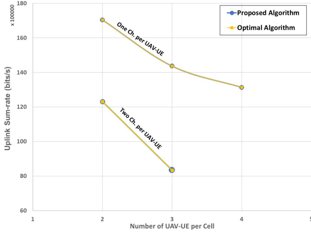
Fig. 8. Comparison with the optimal algorithm.
