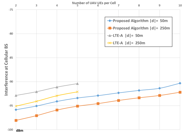
Fig. 5. Interference value at the cellular BS for different schemes in the licensed spectrum vs. n (number of UAV-UEs per cell).
