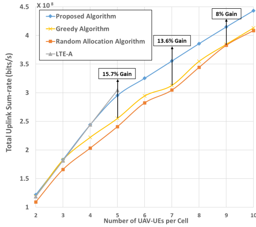
Fig. 3. Total uplink sum-rate as the number of UAV-UEs per cell varies.
