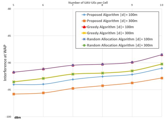
Fig. 6. Interference value at the WAP for different schemes in the unlicensed spectrum vs. n (number of UAV-UEs per cell).
