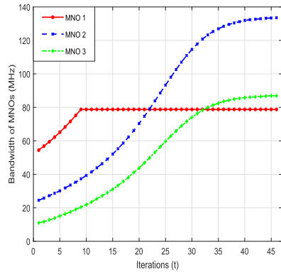
Fig. 8. Variation in the required bandwidths of three MNOs in lightly CA.
