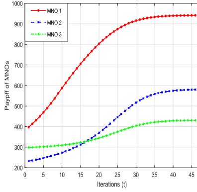
Fig. 6. Payoffs of three MNOs during the iterations of IPA in lightly CA.
