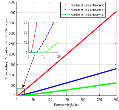
Fig. 5. Coexisting number of IoT devices versus bandwidth.
