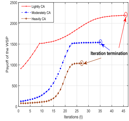
Fig. 9. Variation in the payoff of the WSP.
