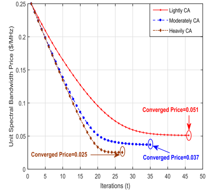
Fig. 10. Variation in the bandwidth price of the WSP.
