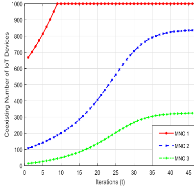
Fig. 7. Variation in the coexisting number of IoT devices for three MNOs in lightly CA.
