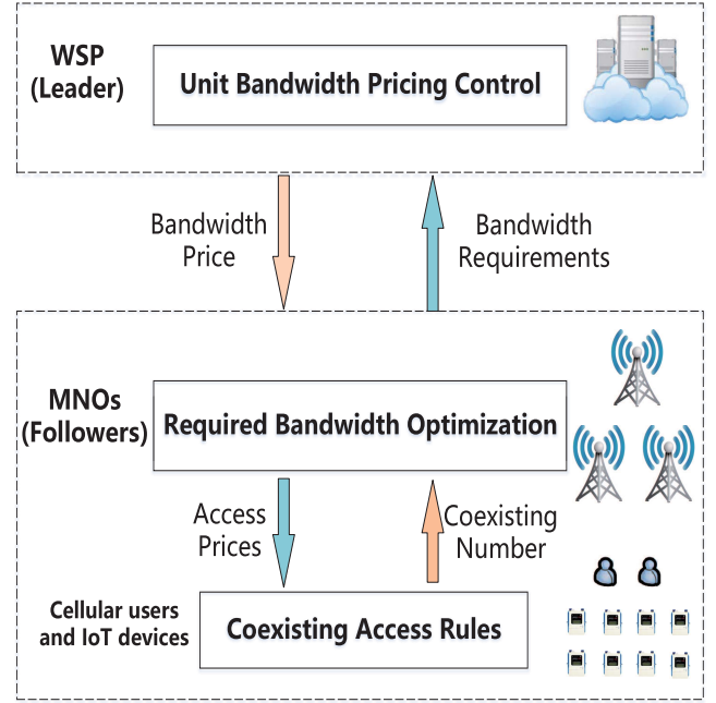
Fig. 2. A Stackelberg pricing game framework for pricing, spectrum sharing, and coexisting access.
