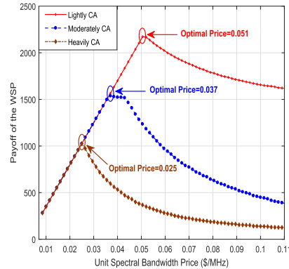
Fig. 11. The payoff of the WSP versus bandwidth price.
