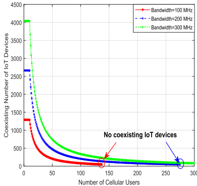
Fig. 4. Coexistence of cellular users and IoT devices at different bandwidths.
