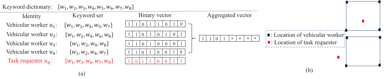
Fig. 4. An example of keyword encoding and all location situations about a task requester and the bounding area of vehicular workers.
