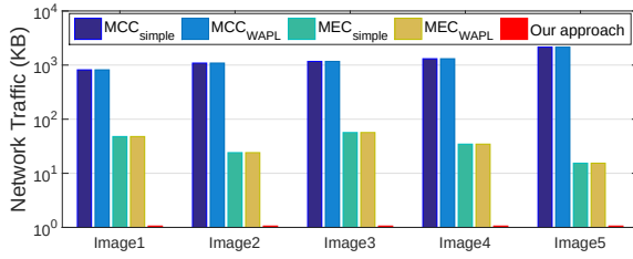
Fig. 9. Network traffic for different approaches.
