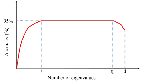
Fig. 4. The contour of Theorem 1. The eigenvalues have been sorted in reverse order. r , q , and d are indexes of eigenvalues. There are r positive eigenvalues, q-r zero eigenvalues, and d-q negative eigenvalues.
