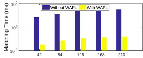
Fig. 11. Matching time for different cases.
