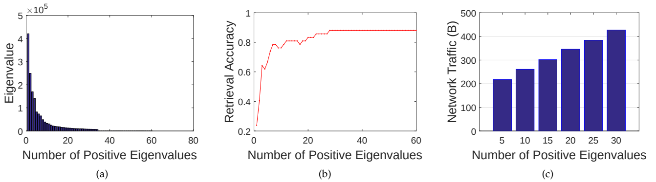
Fig. 13. Relationship between eigenvalue, retrieval accuracy, network traffic and the number of positive eigenvalues
