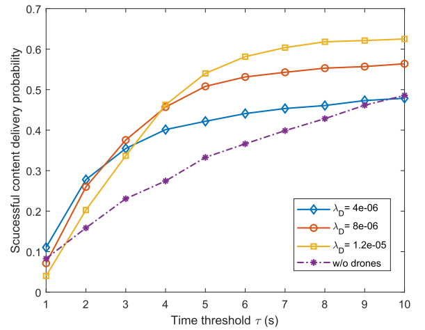
Fig. 6. The total SCD probability with different settings, where Q = 20 Mb, P_m = 25 dBm, H_D = 100 m, \alpha_M = 2.25 , L = 10^3 , K = 6 , and K_d = 2 .
