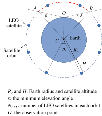
Fig. 7 Illustration of a satellite orbit
