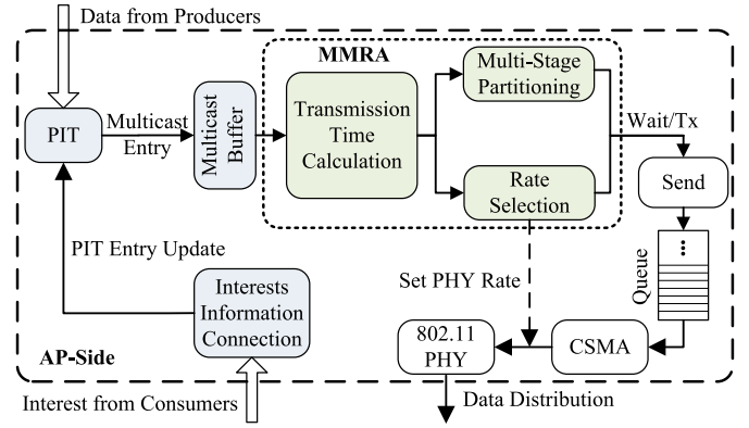
Fig. 4. Overview of NDN-MMRA scheme for WLAN.
