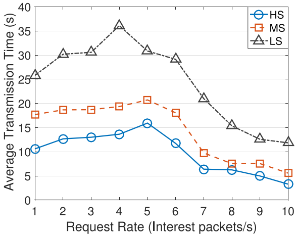
Fig. 11. Impact of the request rate.
