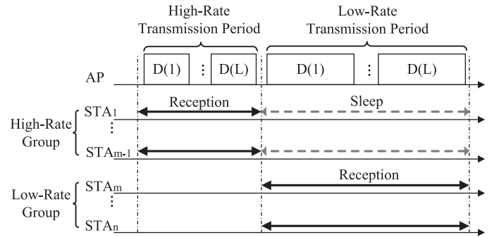
Fig. 7. Multi-rate transmission in a NDN multicast group.
