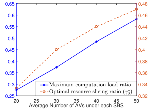
FIGURE 9. Adaptation of maximum computation load ratio and optimal radio resource slicing ratio \gamma_0^* (after Algorithm 2 converges) to different AV traffic load conditions ( \beta = 0.9999 ).
