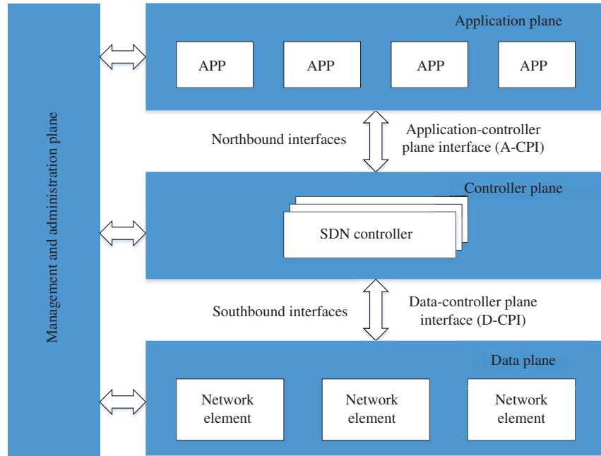
Figure 17 (Color online) A high-level overview of SDN architecture [171].
