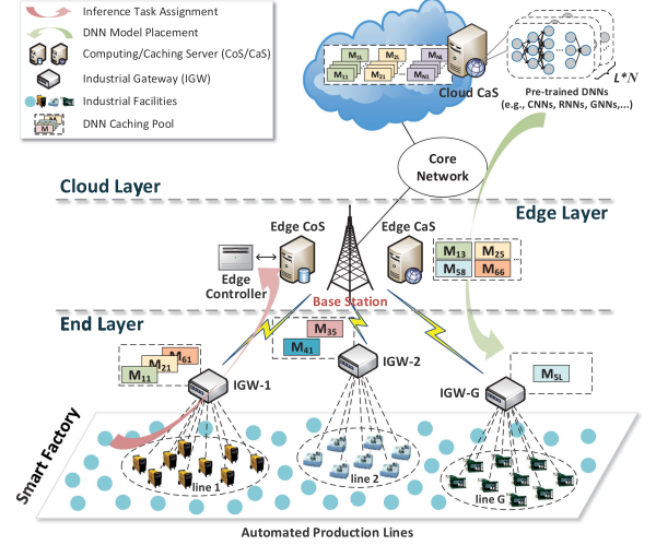
Fig. 2. The end-edge-cloud orchestration architecture in IIoT networks.
