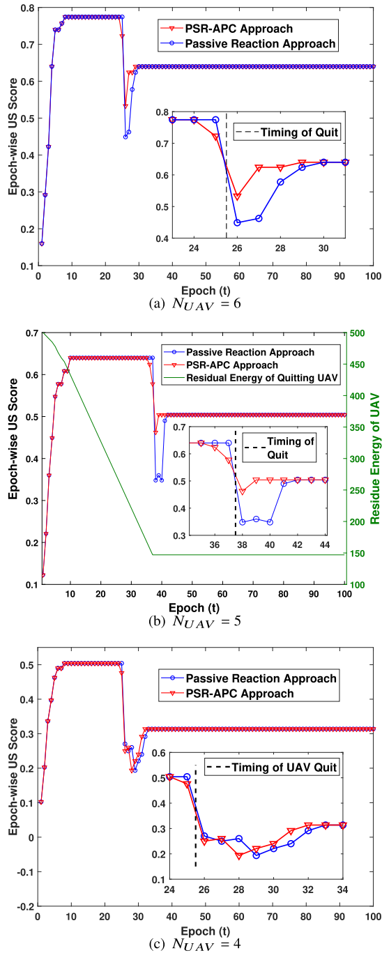
Fig. 7. Case of UAV quit: Epoch-wise reward comparison between the PSR-APC approach and the passive reaction approach.
