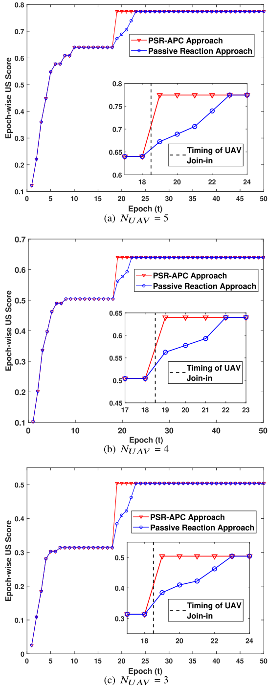
Fig. 9. Case of UAV join-in: Epoch-wise reward comparison between the PSR-APC approach and the passive reaction approach.
