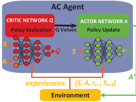
Fig. 2. The diagram for AC method.
