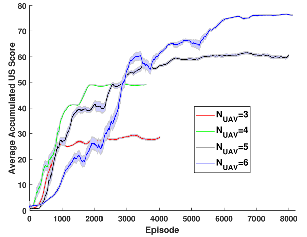
Fig. 5. Convergence with 95% credit interval for different N_{UAV} without UAV or user dynamics as a benchmark.
