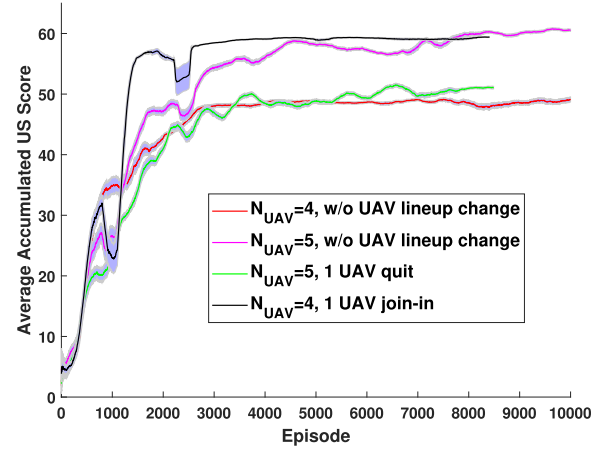
Fig. 11. Convergence with 95% credit interval with user dynamics.
