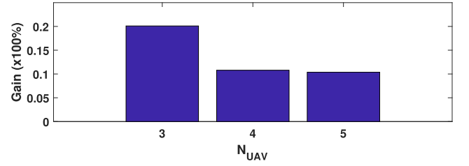
Fig. 10. Case of UAV join-in: Gain (%) of PSR-APC over the passive reaction approach in accumulated US scores during transition to the new optimal UAV positions.
