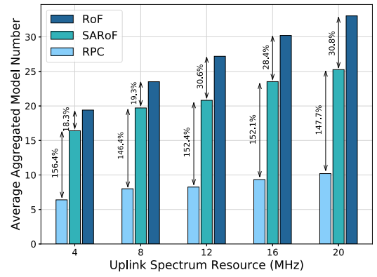
Fig. 10. Average aggregated model number comparison among different schemes with respect to uplink spectrum resource.
