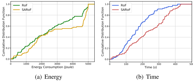
Fig. 12. Cumulative distribution functions of energy consumption and time during the FL process.
