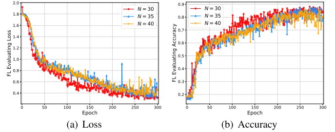
Fig. 7. FL evaluating loss and accuracy with respect to different device (i.e., the IGW) number.
