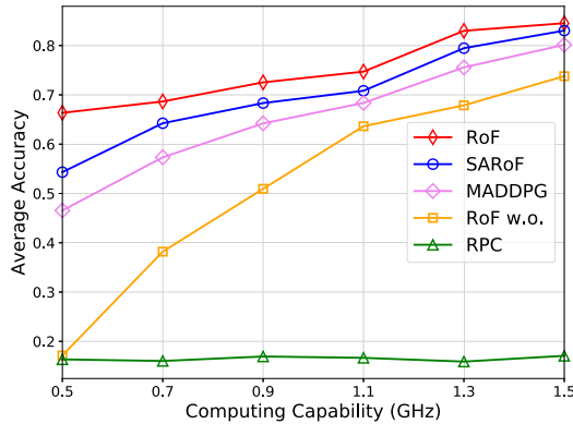
Fig. 9. Average accuracy comparison among different schemes with respect to computing capability.
