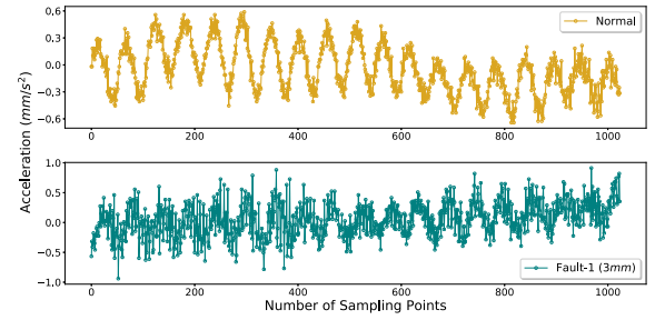
Fig. 4. Two classes of samples in AWE dataset. These two samples are collected from rolling bearings of industrial facilities. “Normal” means the bearing stays in a health condition, and “Fault-1” means the bearing operates under a fault condition with 3 mm severity degree.
