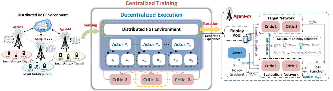
Fig. 2. The architecture of the proposed MASAC-based resource management algorithm.
