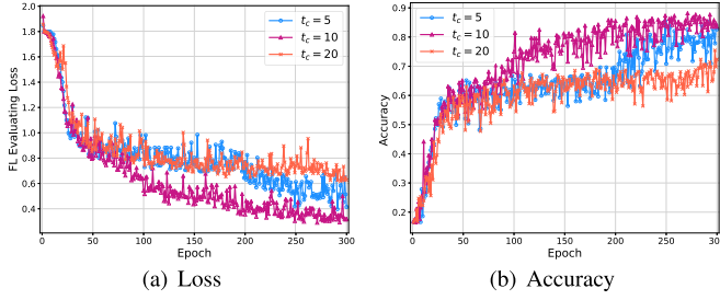
Fig. 5. FL evaluating loss and accuracy with respect to different cloud aggregation frequencies.
