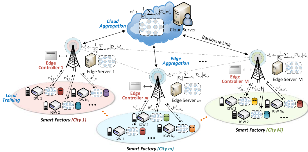
Fig. 1. The three-layer collaborative FL architecture for distributed IIoT networks.
