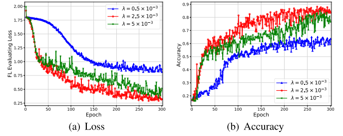
Fig. 6. FL evaluating loss and accuracy with respect to different learning rates.
