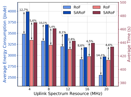
Fig. 11. Average energy consumption and time of different schemes with respect to uplink spectrum resource.
