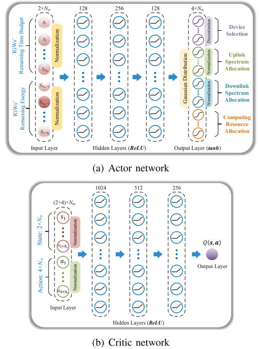
Fig. 3. Actor and critic network structures of MASAC.
