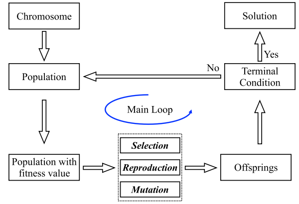
Fig. 3. Procedures of the genetic algorithm.
