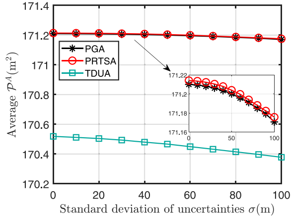
Fig. 11. Average ALAI obtained by different algorithms versus UAVs' position uncertainties (Uniform Distribution).
