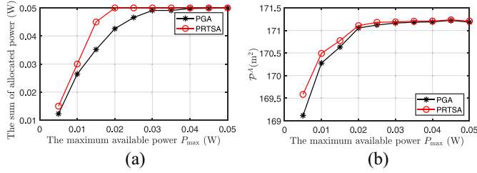
Fig. 8. Comparison of PGA and PRTSA when P_{\max} varies. (a) \|P\|_1 versus P_{\max} . (b) P^A versus P_{\max} .
