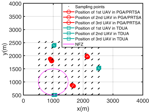
Fig. 15. UAVs' 2-D positions obtained by different algorithms.
