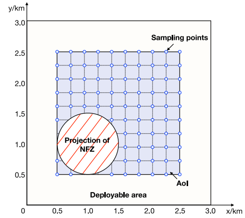
Fig. 2. Two dimensional illustration of the AoI and NFZ.
