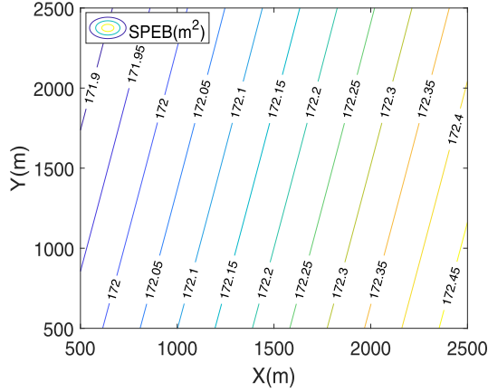
Fig. 4. Distribution of SPEB provided by only satellites.
