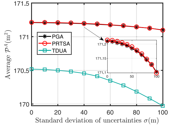
Fig. 12. Average ALAI obtained by different algorithms versus UAVs' position uncertainties (Gaussian Distribution).
