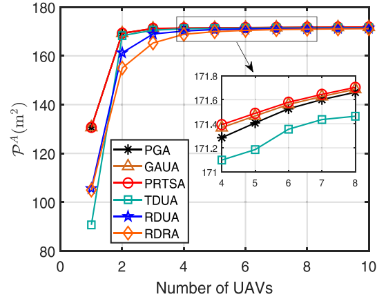
Fig. 5. ALAI versus the number of static UAVs.
