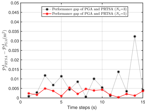
Fig. 14. ALAI gap of PGA and PRTSA algorithms.
