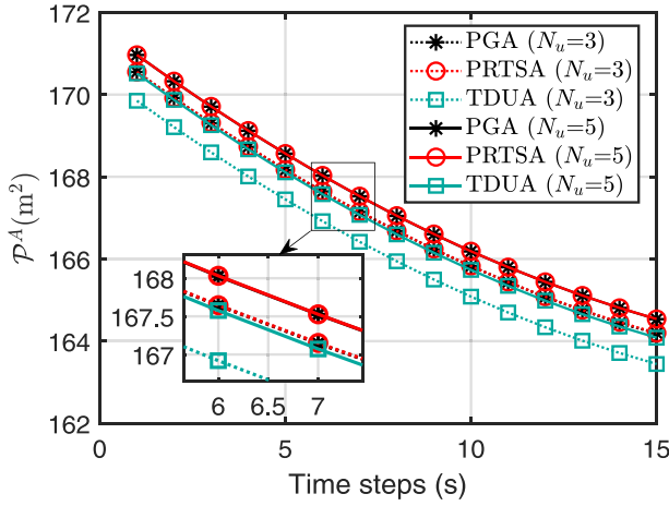
Fig. 13. ALAI solved by different algorithms versus time steps.
