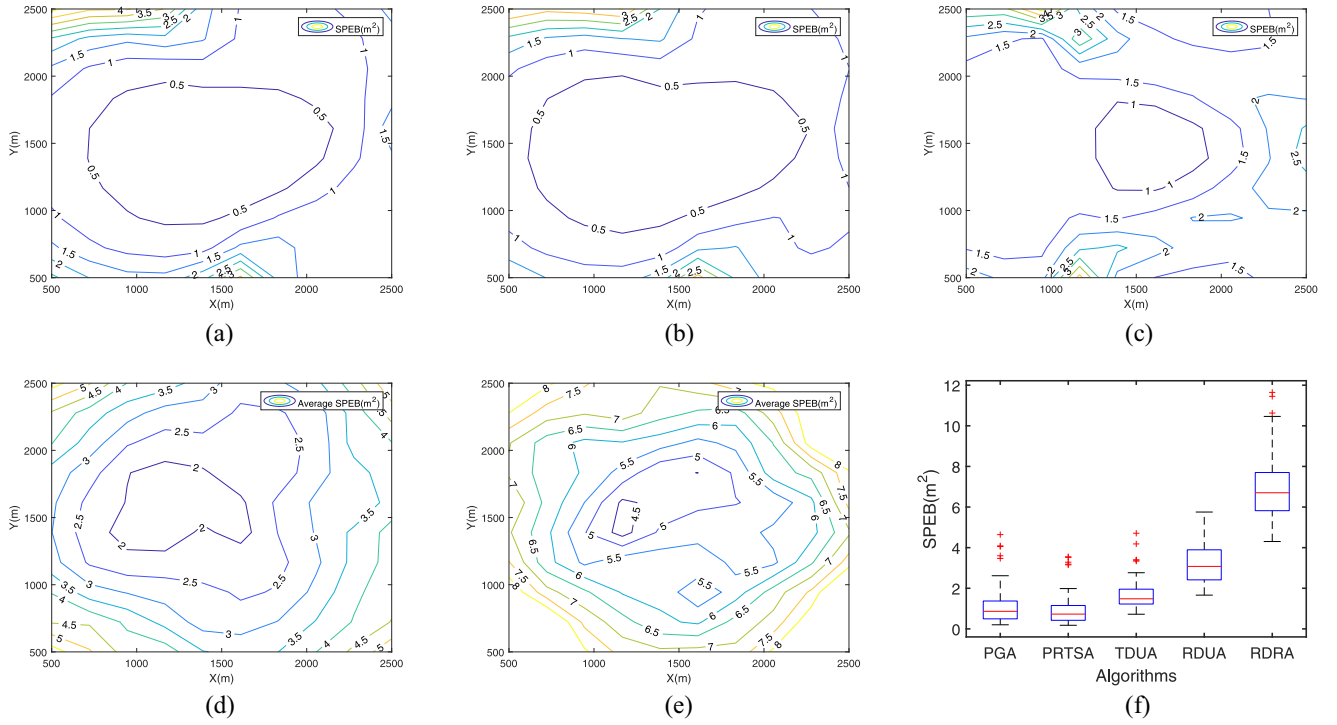
Fig. 10. SPEB distributions of the AoI provided by the static SAILN when using different JPPO algorithms.
