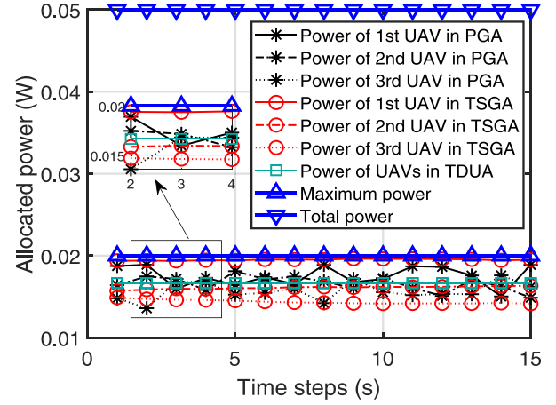
Fig. 16. UAVs' power allocated by different algorithms.
