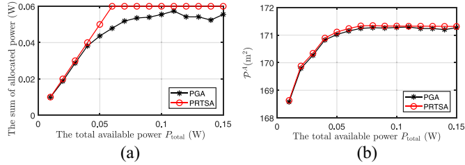
Fig. 9. Comparison of PGA and PRTSA when P_{\text{total}} varies. (a) \|P\|_1 versus P_{\text{total}} . (b) P^A versus P_{\text{total}} .
