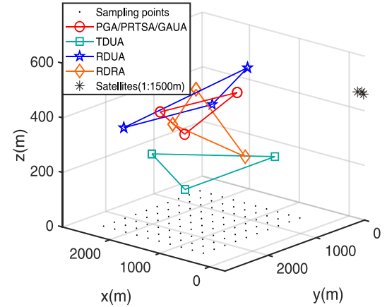
Fig. 6. 3-D positions of static UAVs.
