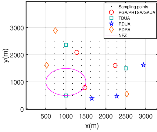
Fig. 7. 2-D positions of static UAVs.
