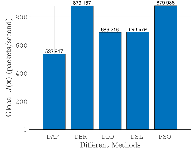
Fig. 9. Performance comparison among different methods.
