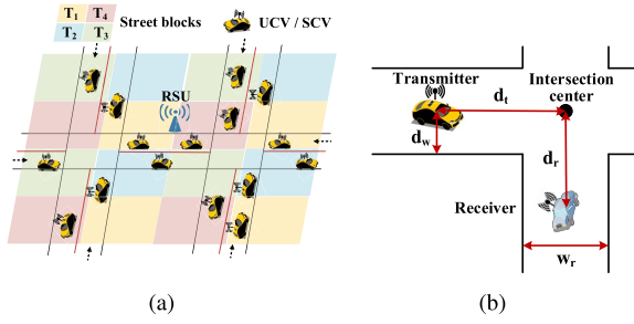
Fig. 2. Illustration of: a) vehicular network; b) NLOS case.
