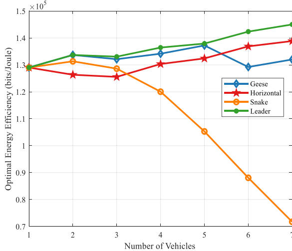
Fig. 8. Total energy efficiency under different forms of vehicle platoons.
