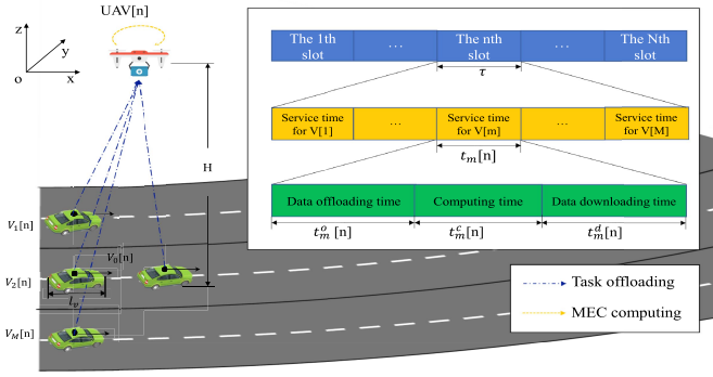
Fig. 1. Typical application scenario of the UAV-MEC assisted turning formation vehicles system. The total service time of each vehicle is the sum of communication and calculation times.
