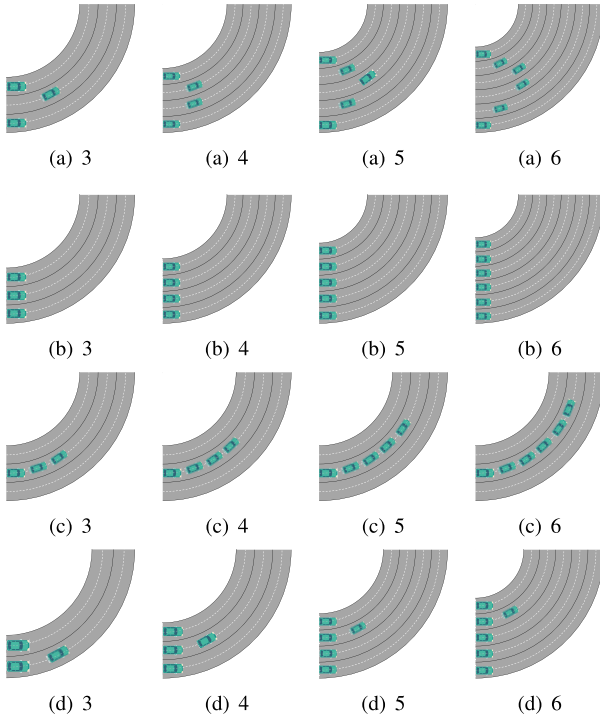
Fig. 7. Four different forms of vehicle formations (number of vehicles varies from 3 to 6). (a) Geese form. (b) Horizontal form. (c) Snake form. (d) Leader form.
