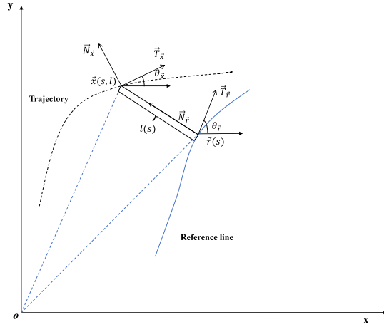
Fig. 2. Schematic of conversion between frenet coordinates and cartesian coordinates.
