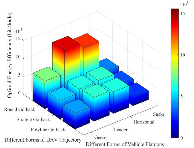
Fig. 9. Total energy efficiency under different forms of vehicle platoons and different forms of UAV trajectories.
