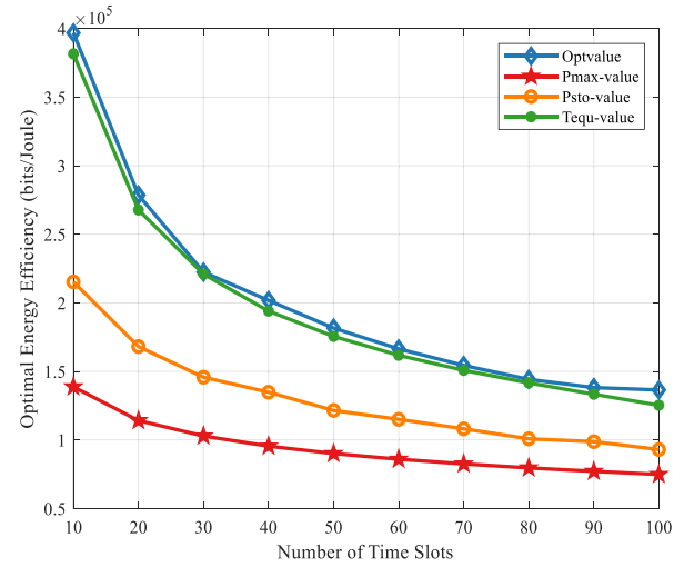
Fig. 6. Total energy efficiency under different number of time slots.
