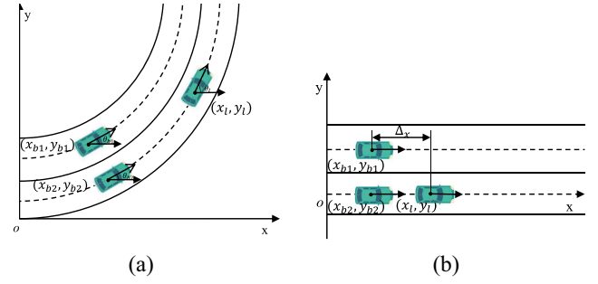
Fig. 3. Platooning vehicles under different coordinate system. (a) Cartesian coordinate system. (b) Frenet coordinate system.
