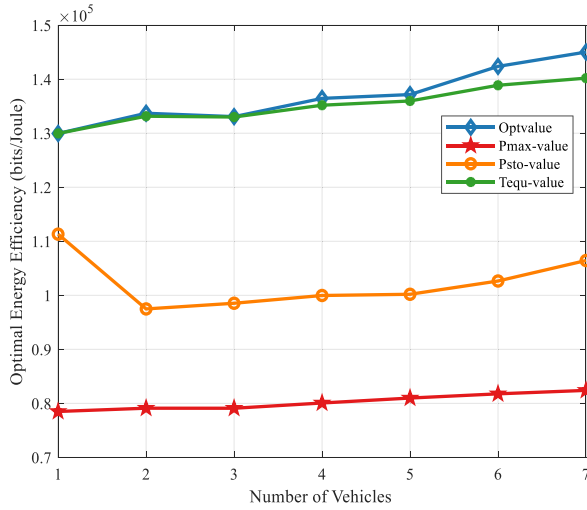
Fig. 4. Total energy efficiency under different number of platooning vehicles.
