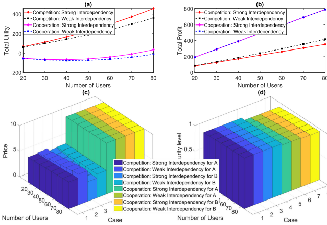
Fig. 8. (a) Total users' utilities, (b) profit, (c) price and (d) security level under competition and cooperation.
