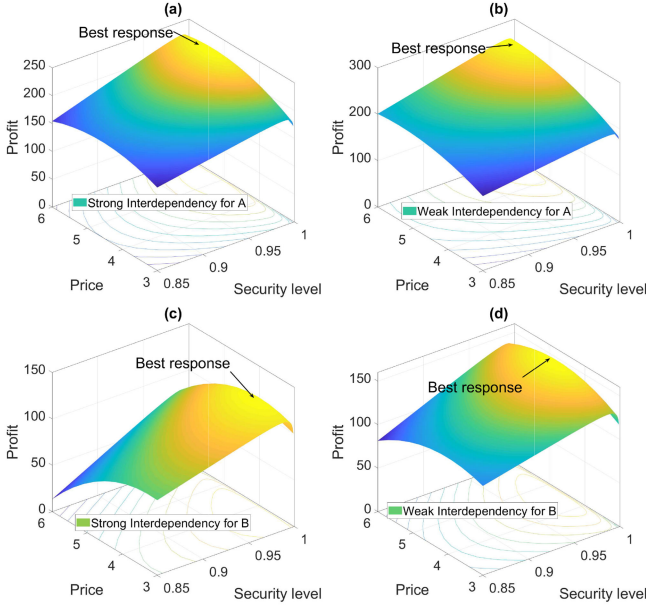
Fig. 3. Best response of the CSSV-A under (a) strong and (b) weak interdependency as well as that of the CSSV-B under (c) strong and (d) weak interdependency.
