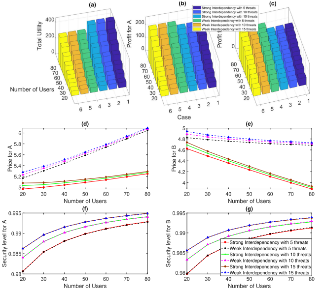
Fig. 9. (a) Total users' utilities, (b) & (c) profit for the CSSVs A & B, (d) & (e) price for the CSSVs A & B, and (f) & (g) security level for the CSSVs A & B with increasing number of the users and increasing numbers of threats.
