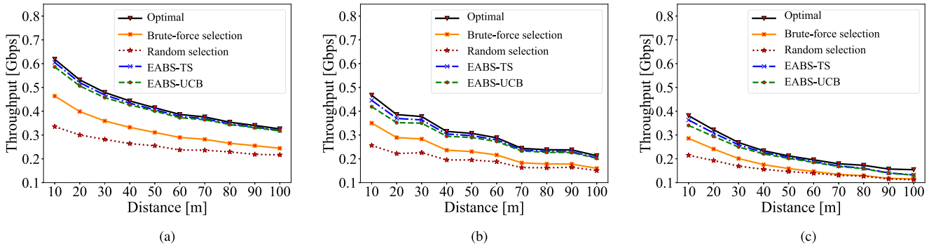
Fig. 4. Throughput comparison for distinct source-destination distances and blockage cases. (a) No blockage scenario. (b) Small blockage scenario. (c) Large blockage scenario.
