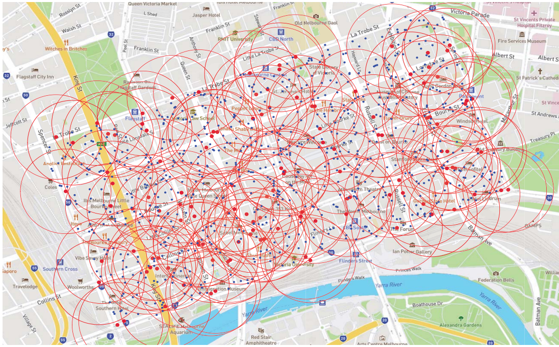
Fig. 2. Distribution of BSs and devices in Melbourne CBD area of Australia.
