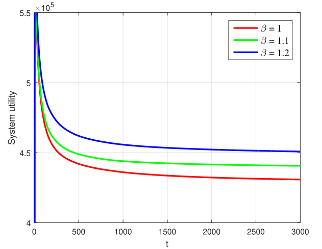
Fig. 5. System utility with different MEC computing capacities.
