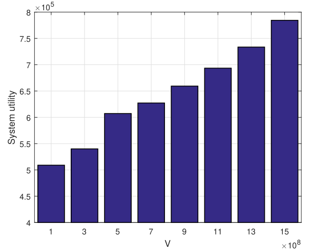
Fig. 1. System utility with different values of V .
