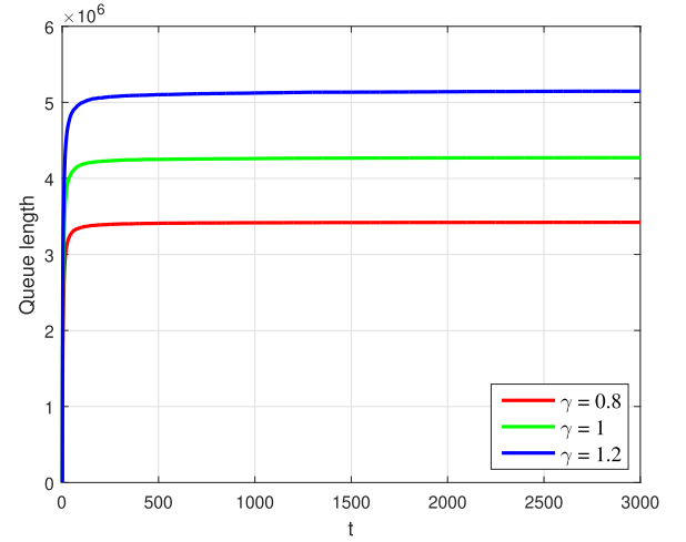
Fig. 4. Queue length with different task arrival rates.
