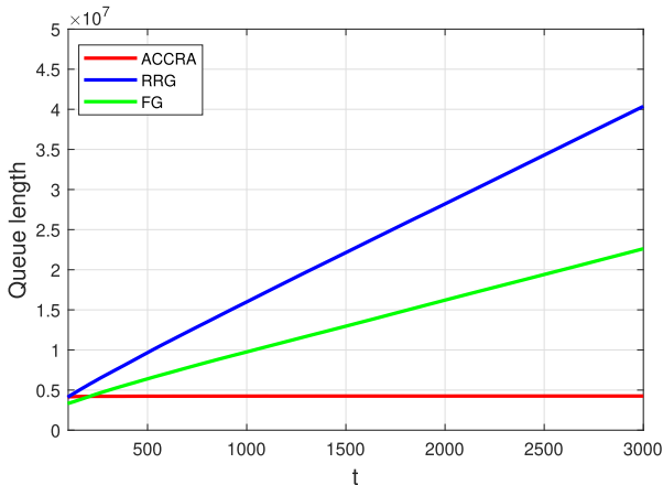
Fig. 8. Queue length with the three different algorithms.
