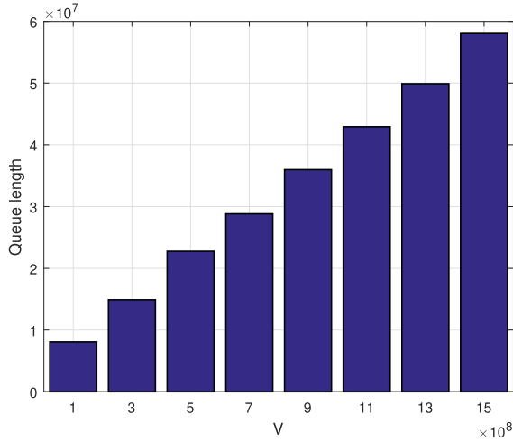
Fig. 2. Queue length with different values of V .
