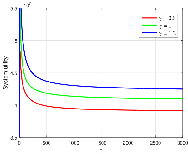
Fig. 3. System utility with different task arrival rates.
