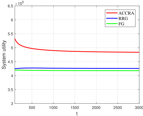
Fig. 7. System utility with the three different algorithms.
