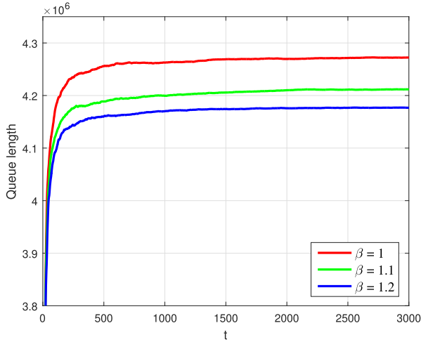
Fig. 6. Queue length with different MEC computing capacities.
