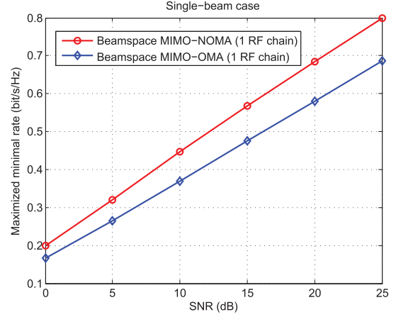
Fig. 2. Max-min rate with respect to the SNR in the single-beam case.
