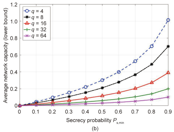
Fig. 7. Average network capacity variation with different requirements on reliable transmission probability and secrecy probability for P_{BS} = 43 dBm, P_{bs} = 30 dBm, L = 8 , and \delta_u = \delta_e = 2 . (a) The impact of the reliable transmission probability requirement on the upper bound of average network capacity with different values of q ; (b) the impact of the secrecy probability requirement on the lower bound of average network capacity with different values of q .
