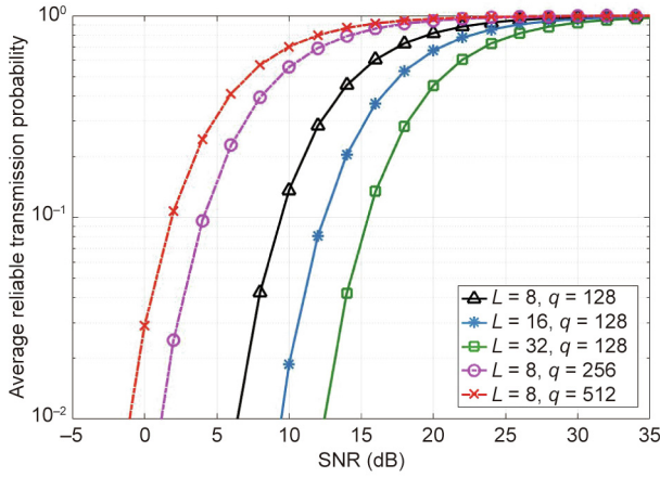
Fig. 5. Average reliable transmission probability variation with SNR under different L and q when \delta_u = 3 .
