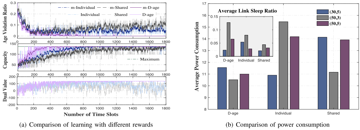
Fig. 6. Comparison of D-age with different scheduling policies.
