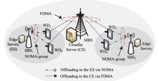
Fig. 1. A two-tier RAN with one MBS and two of SBSs. Each WD offloads parts of its computation-workloads to the MBS and one of the SBSs simultaneously.
