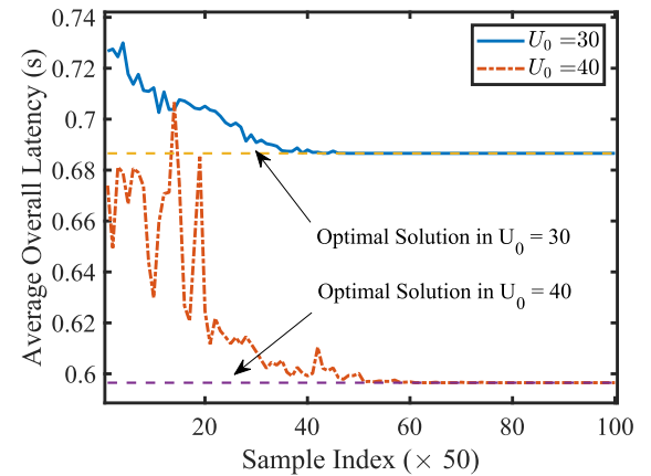
Fig. 7. The effectiveness of CE-based learning Algorithm.
