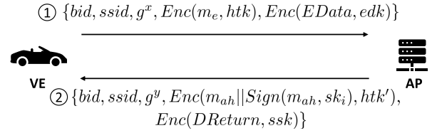
Fig. 3. Anonymous authentication.
