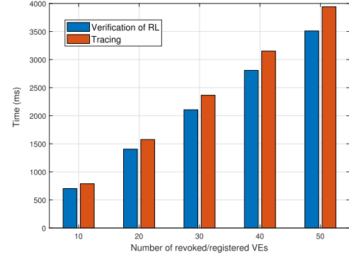
Fig. 6. Computation cost of revocation/tracing.
