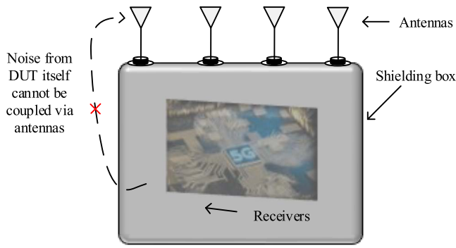
Fig. 10. Noise from the DUT itself cannot be coupled into the receivers via external antennas.
