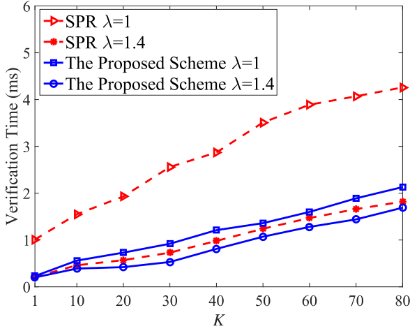
Fig. 7. Verification time of KNN query over NA.
