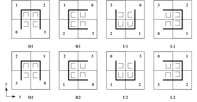
Fig. 2. Fractal rules of Hilbert curve.
