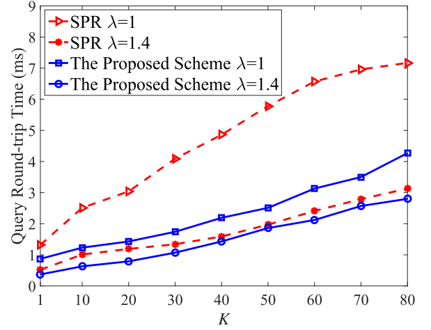
Fig. 9. Round-trip time of KNN query over NA.
