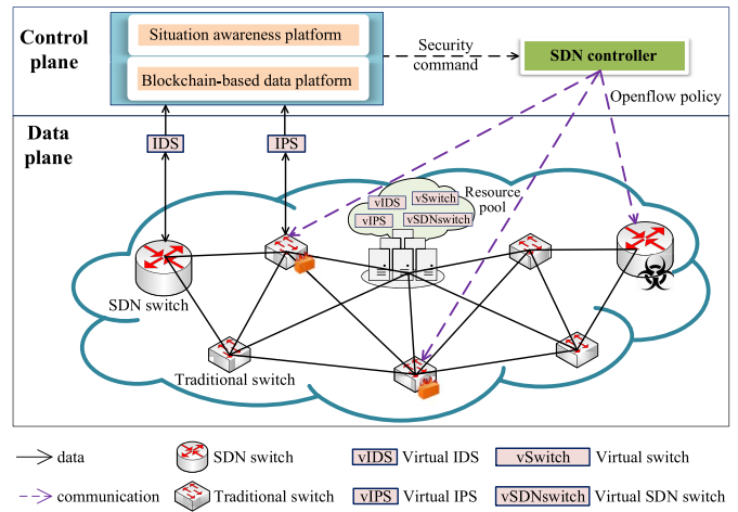
Fig. 22. An example of SDN-based blockchain-IoT architecture. Here, network statistics (e.g., logs) of SDN devices (e.g., SDN switch and traditional switch) can be periodically collected from the data plane by security devices (e.g., intrusion detection system (IDS) and intrusion protection system (IPS)) via a standardized interface such as OpenFlow [4], and then analysed in the situation awareness platform in control plane to detect any network anomalies. Moreover, through network function virtualization (NFV) [154], virtualized network resources (e.g., virtual firewall, virtual IDS, and virtual IPS) can form resource pools and dynamically allocated in accordance with real-time users' demands. Once any anomaly is detected, security commands will be delivered to instruct the controller how to reprogram the data plane for alleviating it.
