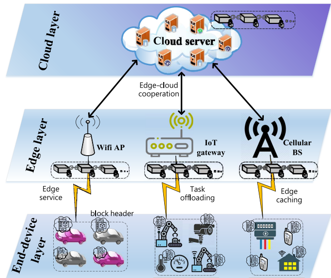
Fig. 11. A typical example of blockchain implementation in ground IoT context under edge-cloud environment.
