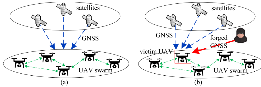
Fig. 18. Illustration of GNSS spoofing attack for UAVs in [134]: (a) normal GNSS operation; (b) GNSS spoofing attack. The detailed workflow of GNSS spoofing attack contains the following steps. ① The adversary tracks the target UAV's GNSS signals and calibrates a forged one with power stronger than that of the legal GNSS signal. ② As legal GNSS signals are suppressed by the forged one, the victim UAV receives the forged GNSS signals and acquires wrong navigation information.
