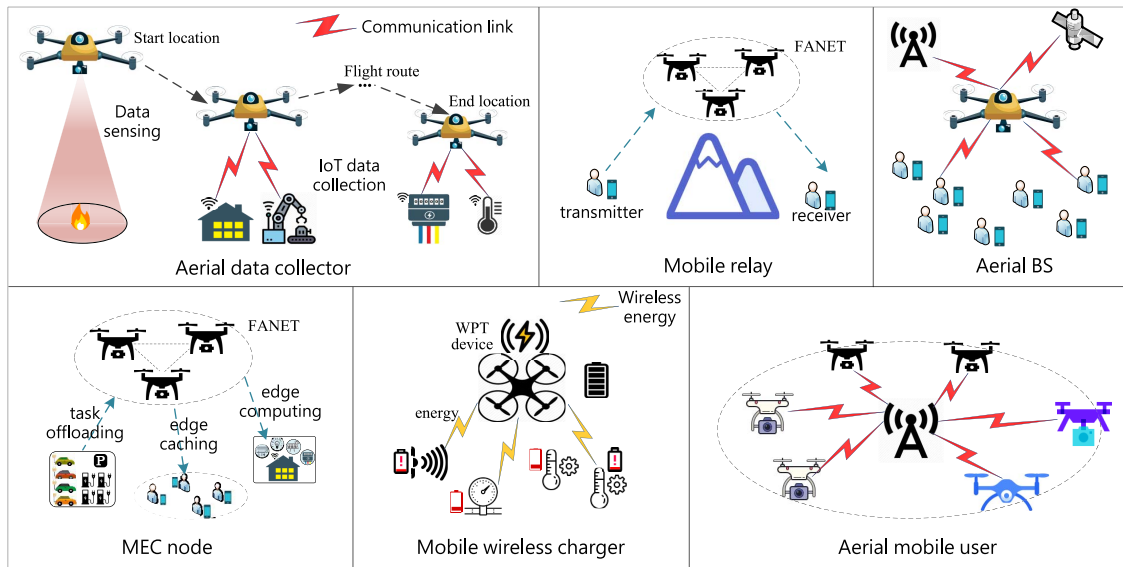
Fig. 10. Typical use cases of UAVs in air-ground integrated networks.
