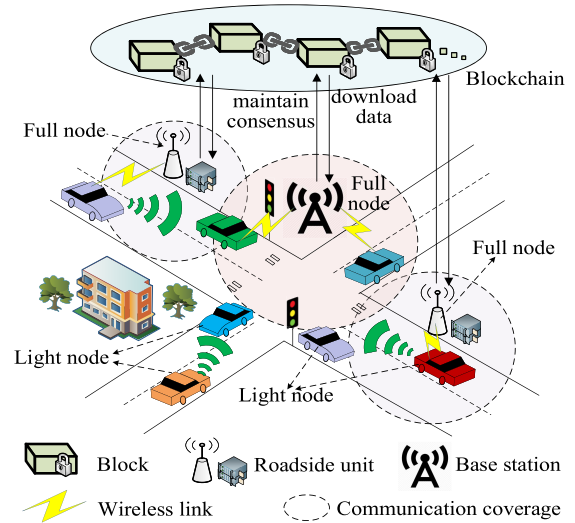
Fig. 7. An example of the implementation of blockchain system in IoV.
