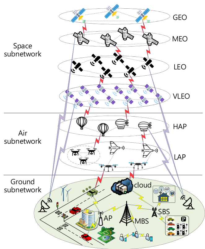
Fig. 2. Architecture of SAG-IoT.
