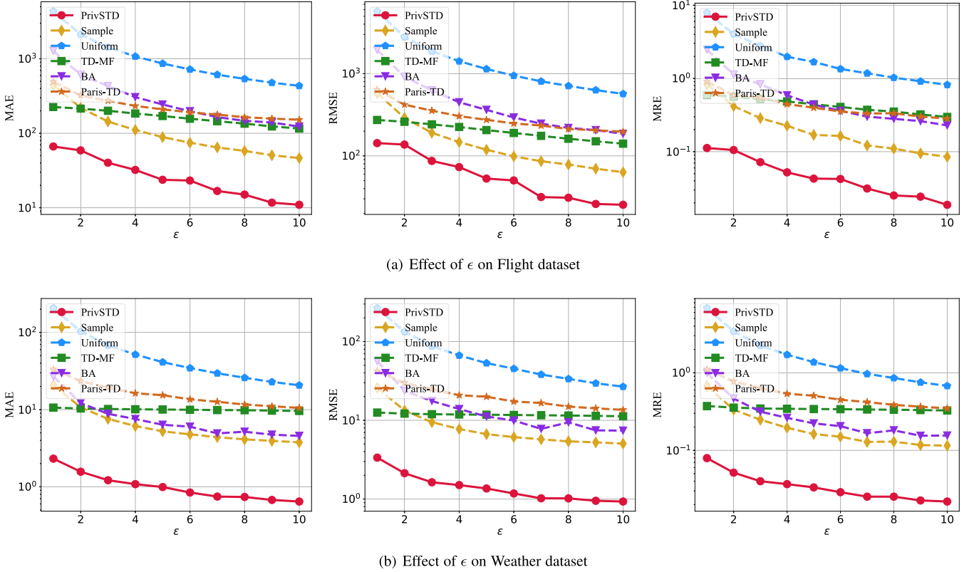
Fig. 9. Effect of privacy budget \epsilon on real-world datasets.
