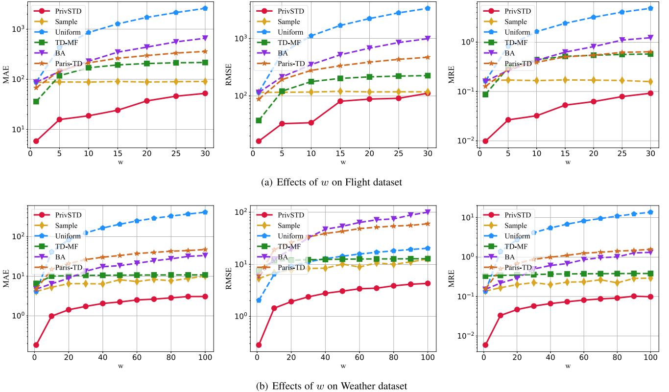
Fig. 8. Effect of sliding window size w on real-world datasets.
