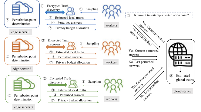
Fig. 1. The framework of PrivSTD.
