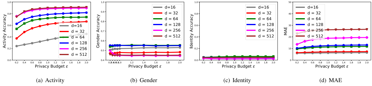
Fig. 9. Effect of encoder-decoder filter of PrivStream-RNN.
