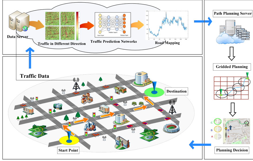
Fig. 1. The scenario of gridded path planning services based on traffic prediction for connected vehicular networks.
