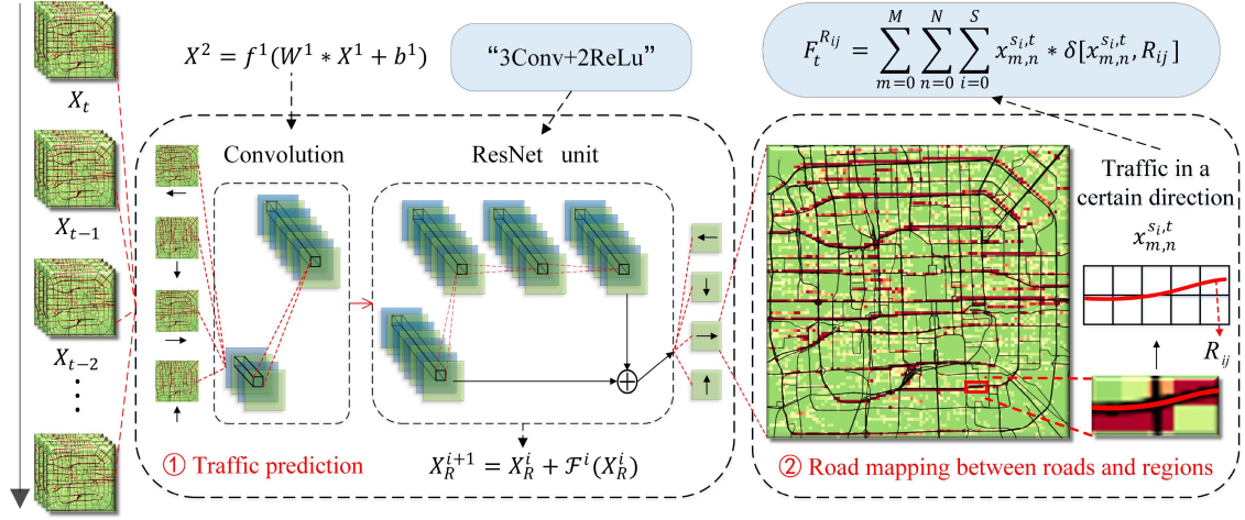
Fig. 4. Neural network architecture and road mapping relationship for regionally fine-grained traffic prediction.
