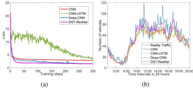
Fig. 6. Comparison of training process and predicted results among different deep learning models.
