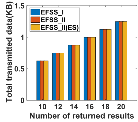
Fig. 8. Communication overhead for returning K results.
