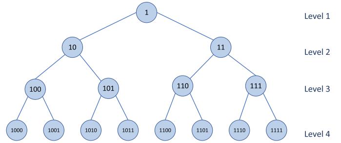
Fig. 2. Hierarchical tree.
