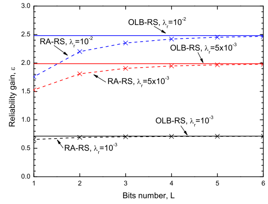
Fig. 7. Reliability gain of the region-based relay selection strategy (RA-RS) as a function of the bit numbers.
