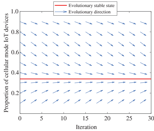
Fig. 7 Direction field of the replicator dynamics
